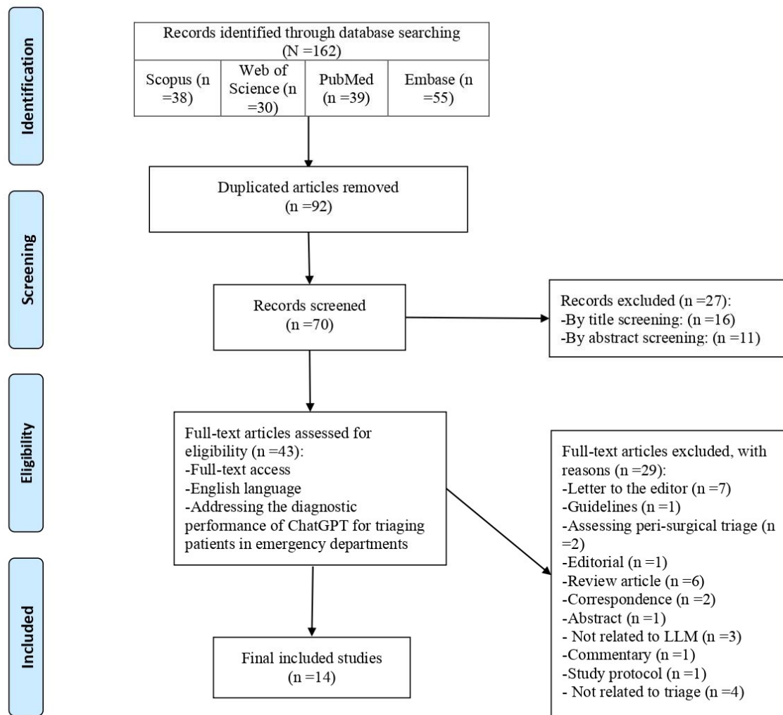
Figure 1. PRISMA Flowchart
