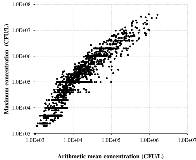
Fig. 3. Relationship between the sample arithmetic mean concentration and the maximum concentration of L. pneumophila in bulk water from 2852 cooling towers in Quebec, Canada.
