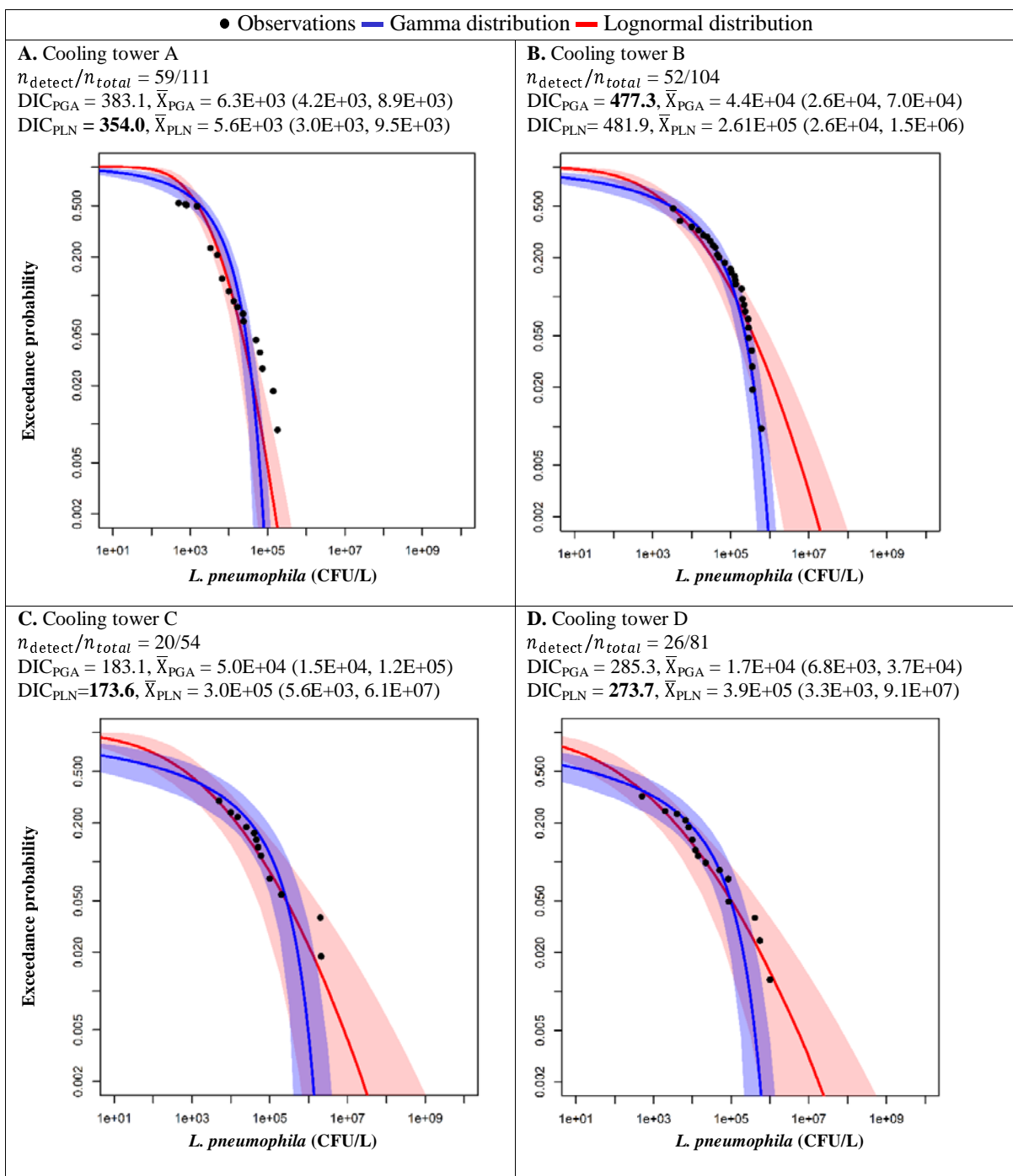
345 Fig. 4. Complementary cumulative distribution function of the Poisson-gamma (PGA) and Poisson 346 lognormal (PLN) distributions fitted to L. pneumophila data from four cooling towers from the Quebec 347 database. The dark blue and red lines represent the best fits of the gamma and lognormal 348 distributions, respectively. The blue and red areas represent the 95% uncertainty intervals of the gamma and lognormal 349 distributions, respectively. The values of the marginal deviance information criterion (mDIC) and the 350 arithmetic mean concentration (with 95% uncertainty interval) in the bulk water of the cooling tower 351 (CFU/L) predicted by each model are listed. mDICs in bold indicate the best-fit models. 352
