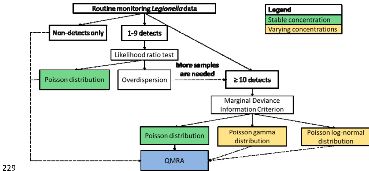
230 Fig 1. Decision algorithm to determine the best fit model to assess L. pneumophila concentrations in bulk 231 water from a cooling tower.
