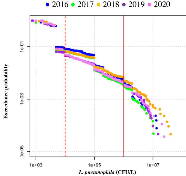
301 Fig. 2. Empirical complementary cumulative distribution function of L. pneumophila concentrations in 302 bulk water from 2852 cooling towers in Quebec, Canada, from 2016 to 2020. The dotted and solid lines 303 indicate concentrations of 10^4 and 10^6 CFU L -1 , respectively.
