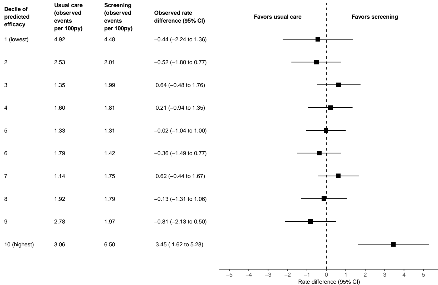
Figure 1: Heterogeneity of Screening Effect using an Effect-based Model
