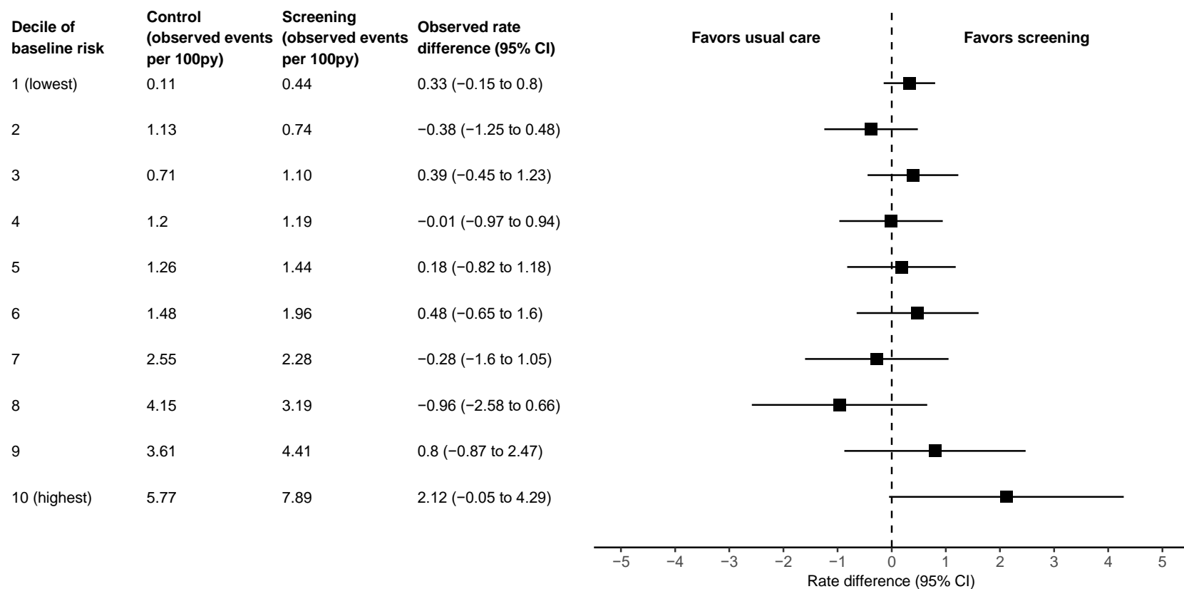
Figure 2: Heterogeneity of Screening Effect using a Risk-based Model
