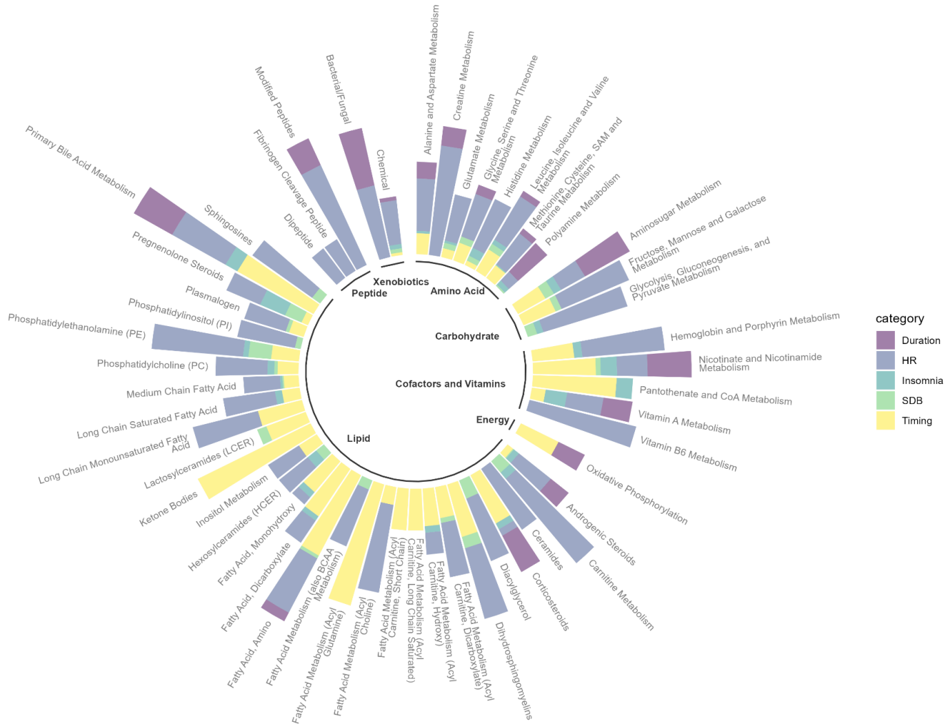
Figure 4. Number of statistically significant associations between metabolites and sleep phenotypes aggregated by subpathway and sleep phenotype domain
