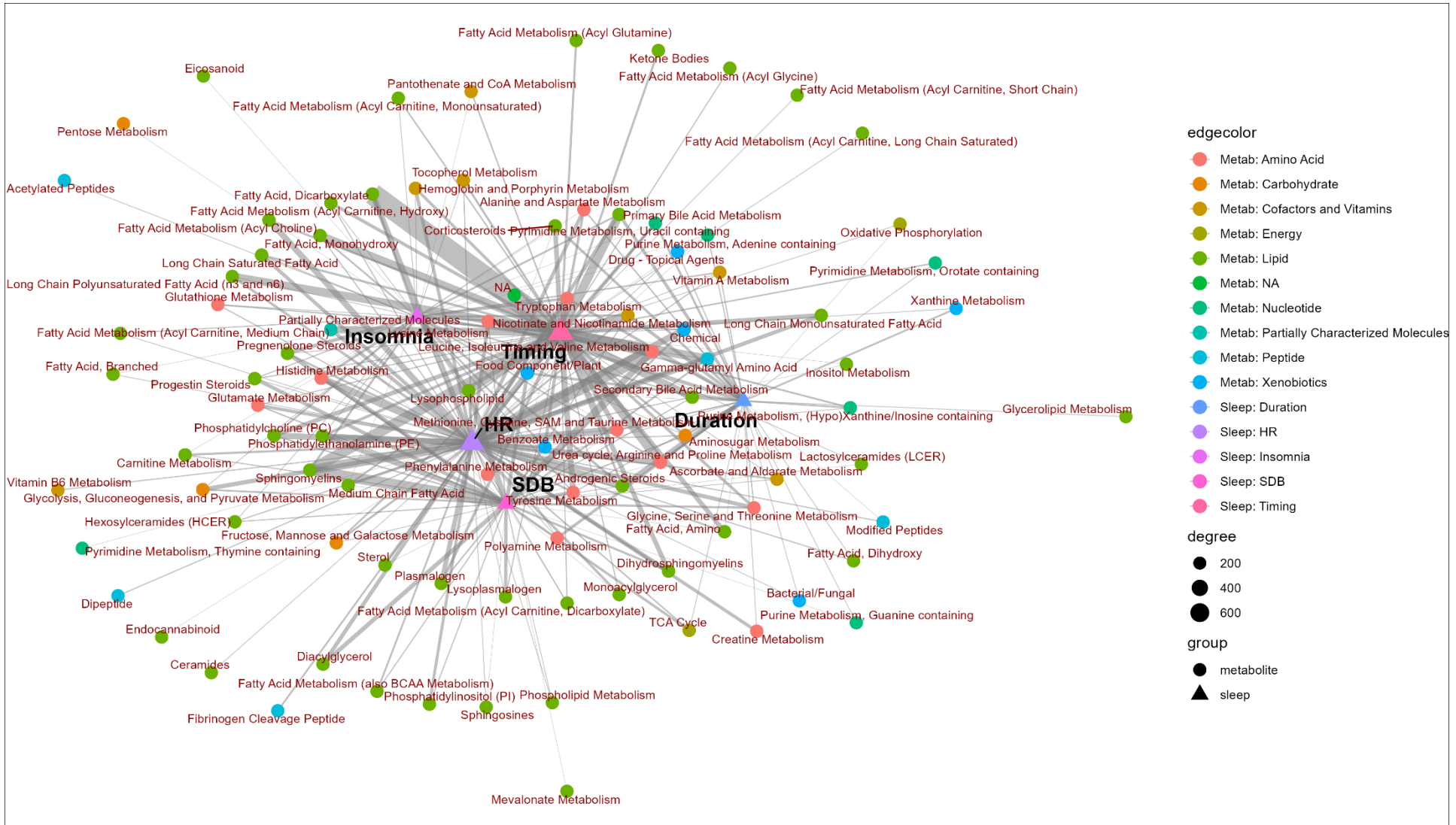
Figure 8. Network based on associations between metabolites and sleep phenotypes aggregated by subpathway and sleep phenotype domain using the Fruchterman-Reingold force-directed algorithm
