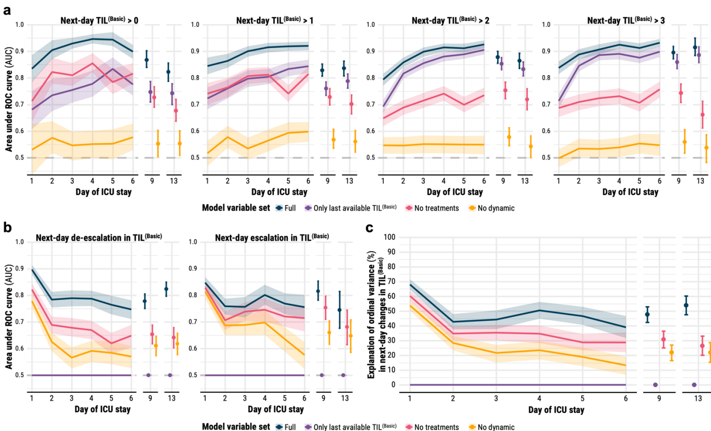
440 Fig. 3. Differential performance in discriminating and explaining next-day TIL (Basic) . All shaded regions 441 surrounding curves and error bars are 95% confidence intervals derived using bias-corrected bootstrapping 442 (1,000 resamples) to represent the variation across 20 repeated five-fold cross-validation partitions. (a) 443 Discrimination performance in prediction of next-day TIL (Basic) – measured by AUC at each threshold of 444 TIL (Basic) – by models trained on different variable sets. The violet line represents the performance achieved 445 by simply carrying the last available TIL (Basic) forward to account for the effect of day-to-day stasis in TIL (Basic) 446 on prediction. The horizontal dashed line (AUC=0.5) represents the performance of uninformative 447 prediction. (b) Discrimination performance in prediction of next-day de-escalation or escalation in TIL (Basic) 448 – measured by AUC – by models trained on different variable sets. The horizontal dashed line (AUC=0.5) 449 represents the performance of uninformative prediction. (c) Explanation of ordinal variation in next-day 450 changes in TIL (Basic) – measured by Somers' D_{xy} – by models trained on different variable sets. 451 Abbreviations: AUC=area under the receiver operating characteristic (ROC) curve, ICU=intensive care unit, 452 TIL=Therapy Intensity Level, TIL (Basic) =condensed, five-category TIL scale as defined in Table 1.
