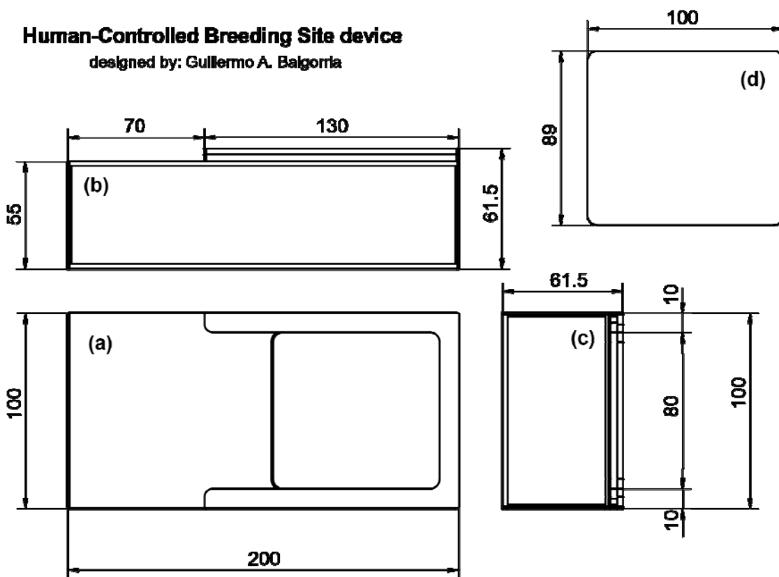
3 Figure 1: Design drawings of the HCBS device, showing (a) top view of the body, (b) side view 4 of the body, (c) front view of the body, and (d) top view of the slicing cap. Measurements are in 5 millimeters (mm).
