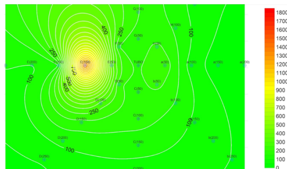
Figure 5. Graphic reconstruction of isodose distribution at level 1.
