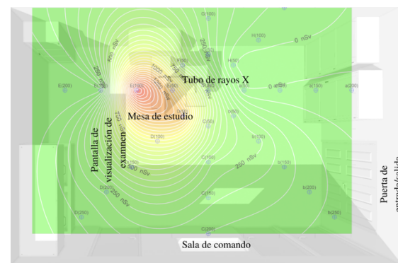
Figure 6. Graphic reconstruction of isodose distribution representing the layout of the room.
