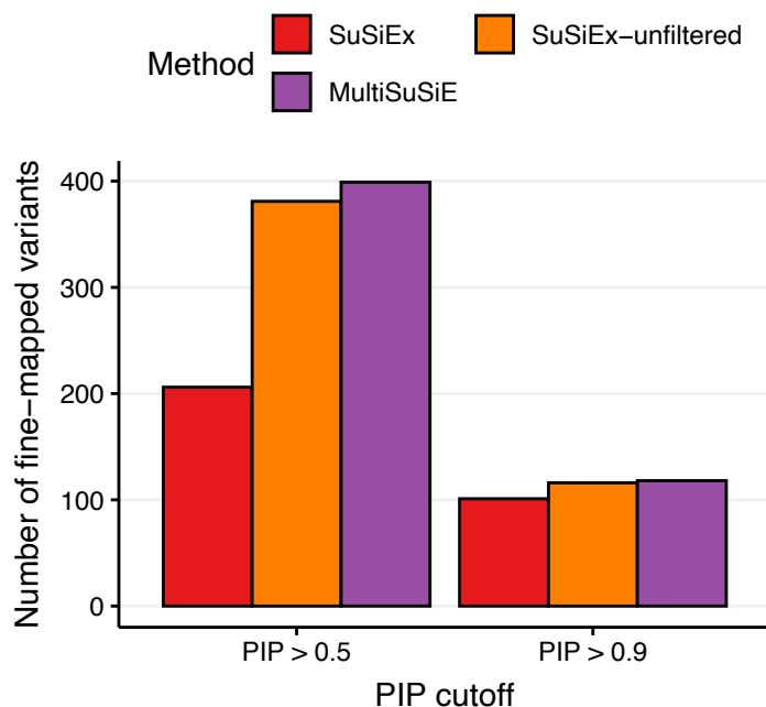
Supplementary Figure 29: Real trait results for Afr47k+Eur47k across fine-mapping methods including SuSiEx-unfiltered. We report the number of variant-trait pairs with PIP > 0.5 or 0.9 across 14 uncorrelated traits using Afr47k+Eur47k.
