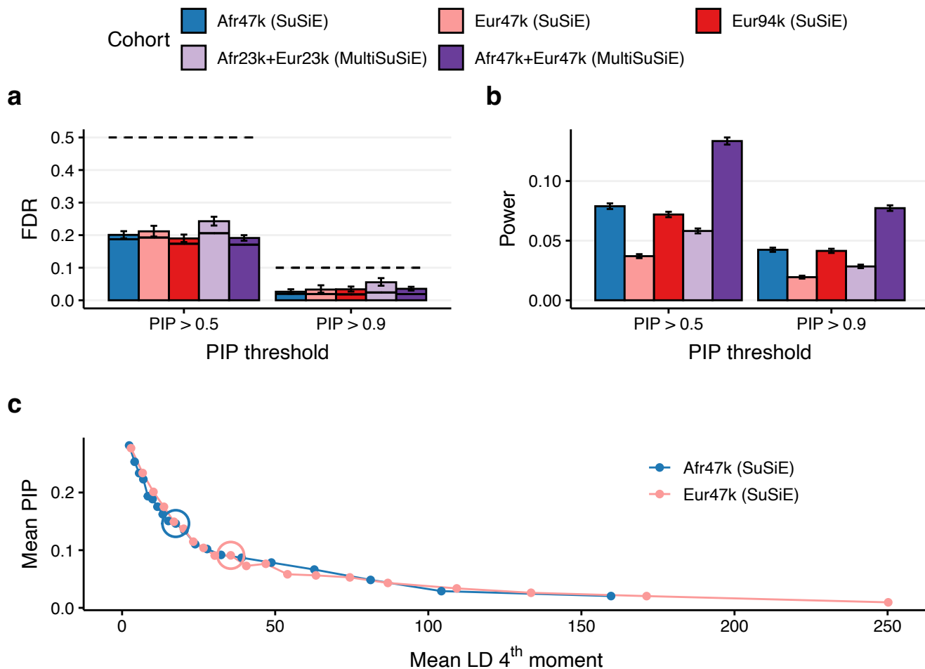
Figure 1: Simulation results across ancestries and sample sizes analyzed. We report (a) the FDR (bars), conservative FDR upper bound (dashed line), and expected FDR (solid bars) at PIP > 0.5 and PIP > 0.9, (b) power at PIP > 0.5 and PIP > 0.9, (c) mean PIP of causal variants with MAF > .05 within 20 equally sized LD 4 th moment bins in Afr47k and Eur47k fine-mapping. Error bars denote 95% confidence intervals. Circled dots denote the 10 th LD 4 th moment bin for each cohort. Numerical results are reported in Supplementary Tables 2-3.
