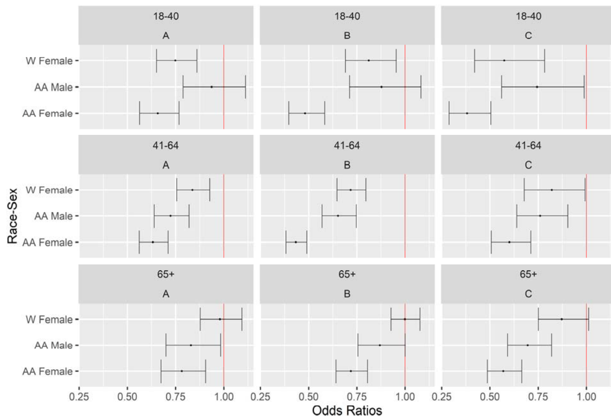
Figure 3 Odds ratio plots with 95% CIs for the Race-Sex variable for patients split by age group at each ED, with the reference level being White men. Each row corresponds to a different age group and each column is an ED.
