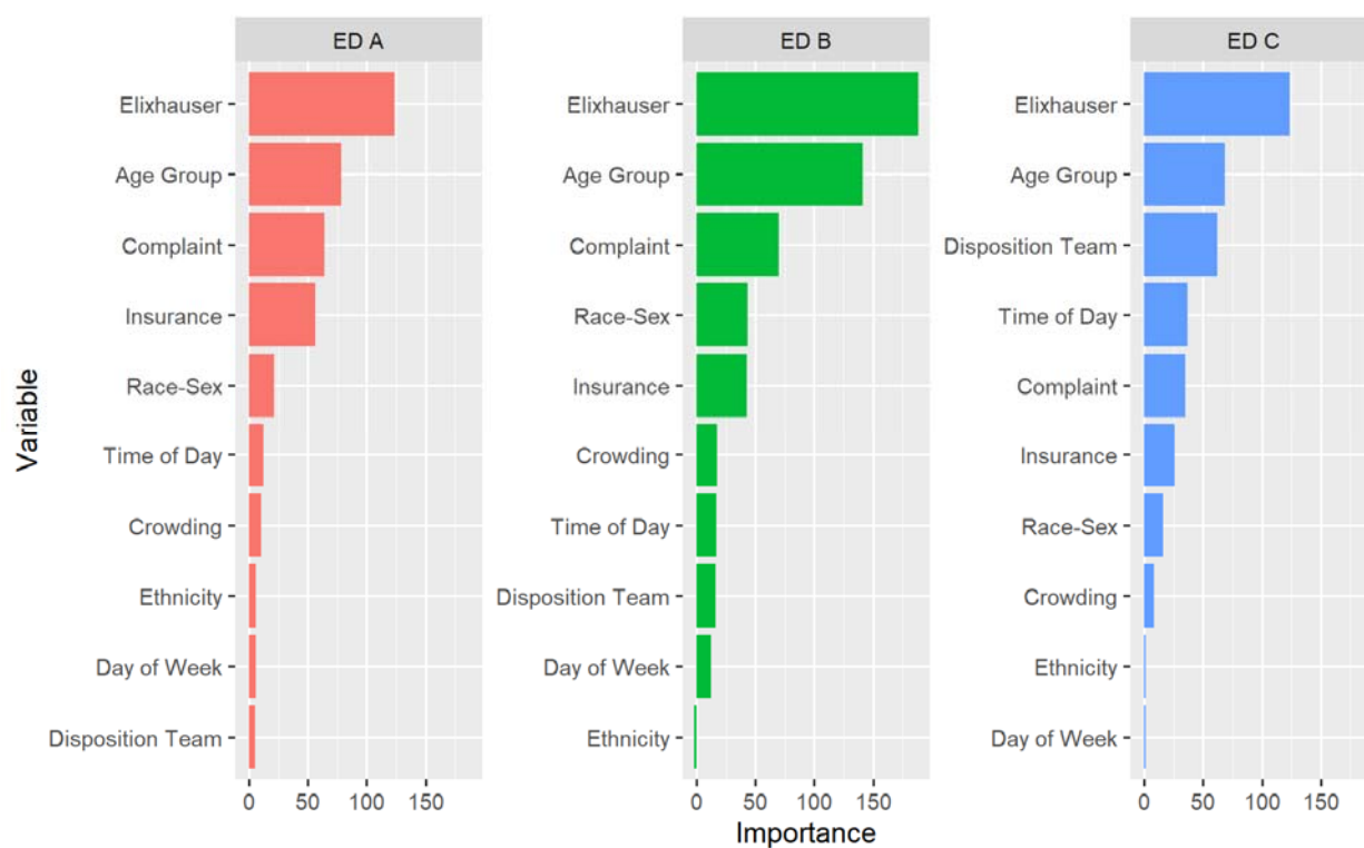
Figure 1 Variable importance plots based off mean decrease in accuracy for the three different random forests associated with the three EDs.
