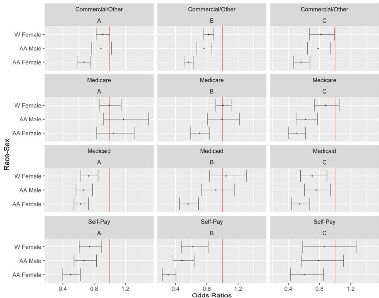
Figure 4 Odds ratio plots with 95% CIs for the Race-Sex variable for patients split by insurance status at each ED, with the reference level being White men. Each row corresponds to a different insurance group and each column is an ED.
