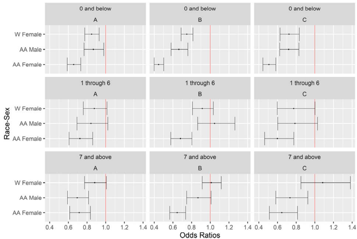
Figure 2 Odds ratio plots with 95% CIs for the Race-Sex variable for patients split by Elixhauser score at each ED, with the reference level being White men. Each row corresponds to a range of Elixhauser scores, and each column is an ED. On the vertical axis labels, AA means African-American, and W means White.
