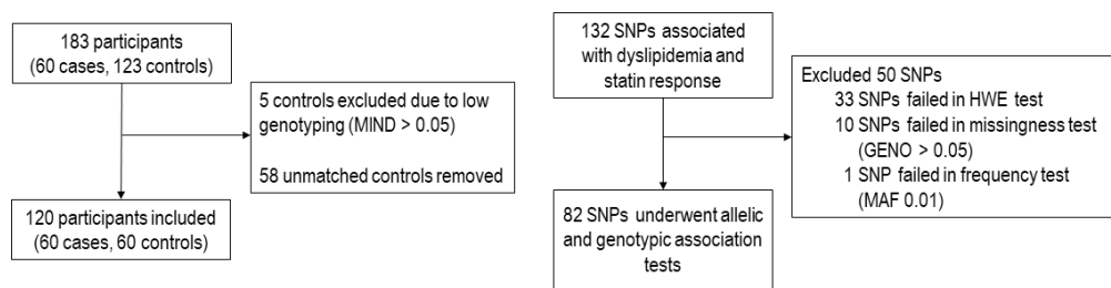
167 FIG 1. Schematic diagram of data processing and analysis for the high LDL-C group. A total 168 of 183 participants (A) and 132 SNPs (B) were analyzed to determine the association of genetic 169 variants with high LDL-C and lipid metabolism. Abbreviations: MIND – individual missingness; 170 SNP – single nucleotide polymorphism; HWE – Hardy-Weinberg equilibrium; GENO – genotypic 171 missingness 172
