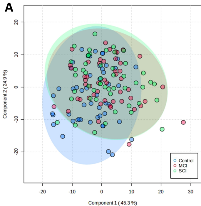
Scores Plot
