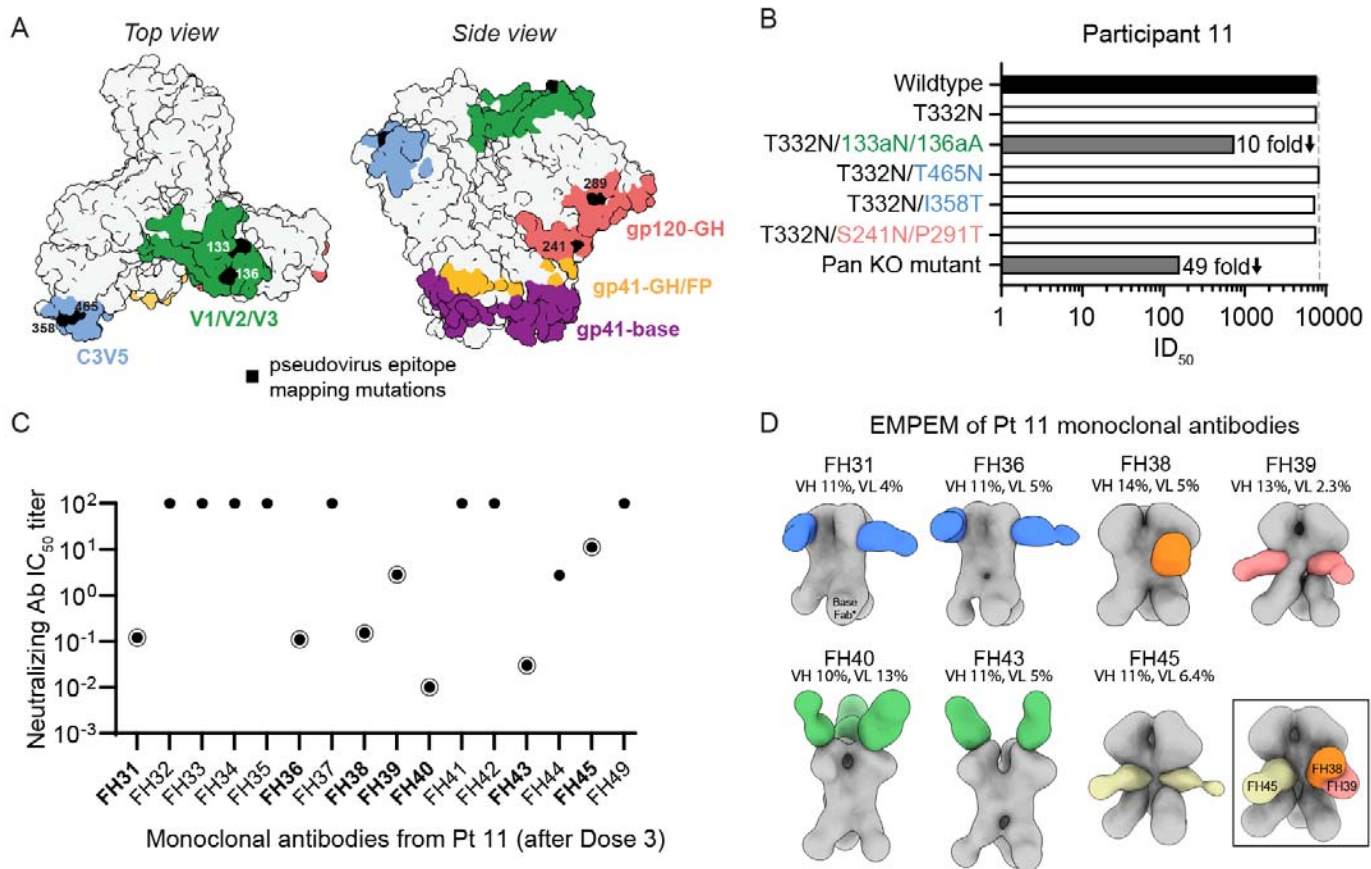
Figure 5. Mapping BG505 SOSIP.664 gp140 epitope regions recognized by serum and monoclonal neutralizing antibody responses. (A) Schematic representation of the epitope surface targeted by polyclonal serum antibodies to BG505 SOSIP.664 gp140, as determined by published cryo-EM structures (Antanasijevic et al., 2021). The location of mutations used in pseudovirus-based epitope mapping are marked at indicated positions. (B) Serum antibody neutralization titers for participant 11 were mapped using pseudoviruses with mutations introduced at indicated positions and color coded as in A. “Pan KO mutant” includes the following mutations: T332N, T465N, S241N, 133aA, and 141aA. Open bars represent titers that were not impacted by the mutations (<three-fold reduction relative to wildtype BG505 virus). (C) IC 50 of monoclonal antibodies against BG505/T332N isolated from Participant 11 after third dose. Circled points indicate samples also analyzed by EMPEM. (D) EMPEM of indicated monoclonal antibodies with % somatic hypermutation of heavy and light chains indicated.
