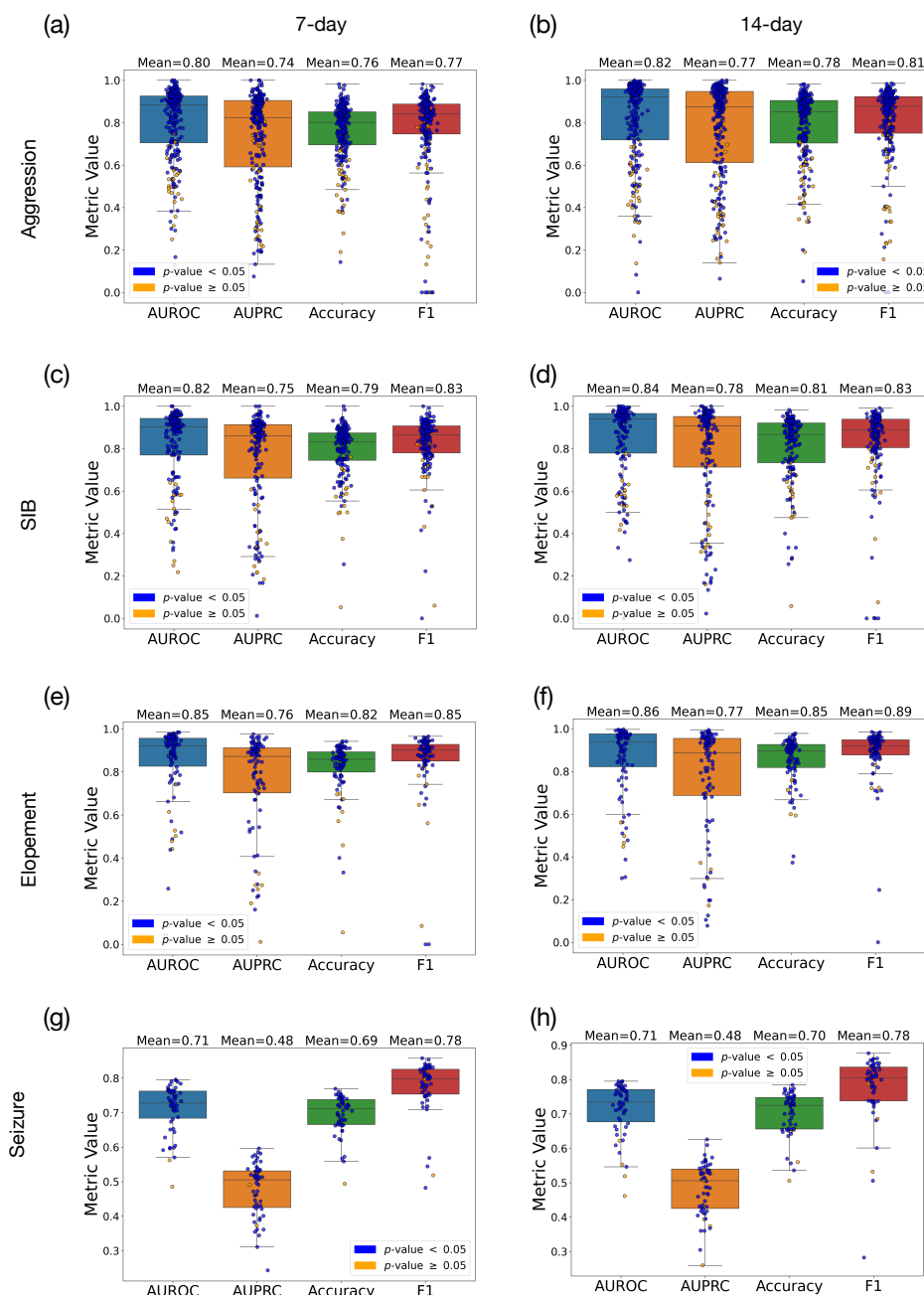
Figure 5: Representation of prediction results using 7-day and 14-day spans of prior historical data for predicting SIB, elopement, and seizure, presenting AUROC, AUPRC, accuracy, and F1 score. Blue and yellow circles represent cases where we achieved, and could not achieve, statistical significance, respectively. Subfigures (a), (c), (e), and (g) depict the results for aggression, SIB, elopement, and seizure using 7-day data, while (b), (d), (f), and (h) illustrate the results for SIB, elopement, and seizure using 14-day data.
