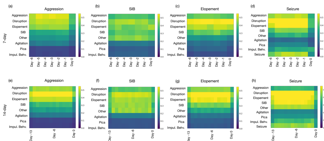
Figure 4: Representation of features importance using GradCAM for predicting high-risk events. Day -j refers to the j^{th} day preceding the target day for which the prediction is being made. (a), (b), (c), and (d) illustrate the feature importance rankings for predicting aggression, SIB, elopement, and seizures, respectively, based on a 7-day window. (e), (f), (g), and (h) extend the analysis to a 14-day window for the same outcomes. The comparison highlights how the predictive value of specific features shifts with the extension of the historical data period.
