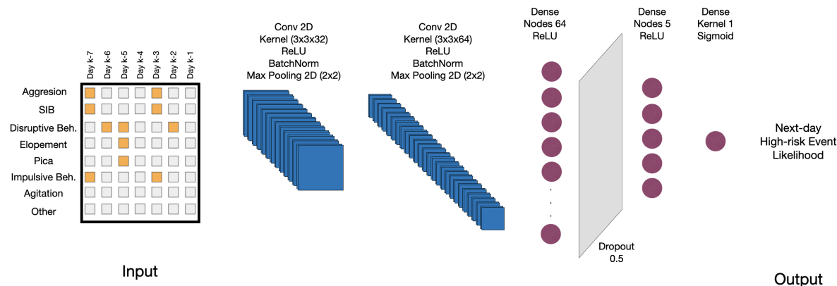
Figure 2: The diagram illustrates the deep learning model designed for the binary prediction of the occurrence of high-risk behavioral and medical events on the following day. The model architecture includes two-dimensional convolutional layers, batch normalization, max pooling, dense layers with ReLU activation, a dropout layer for regularization, and a final dense layer with a sigmoid activation function for outputting the likelihood for an individual displaying a given behavior (e.g., self-injurious behavior, elopement, or seizure episode) the following day.
