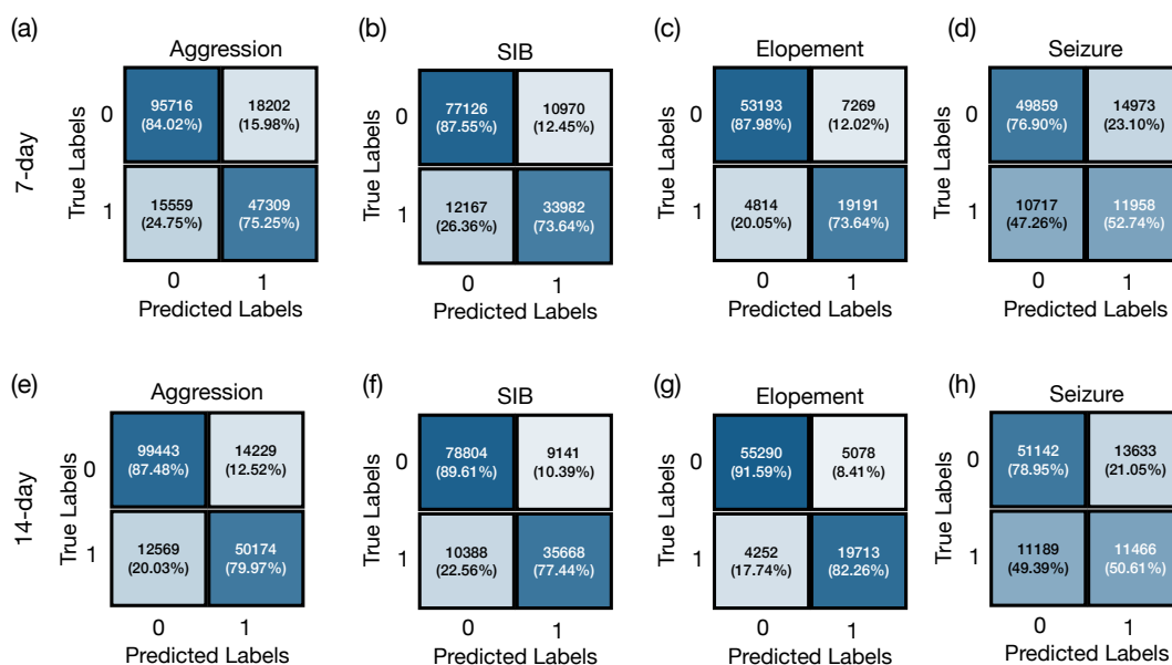
Figure 3: Confusion matrices for predicting aggression, self-injurious behavior (SIB), elopement, and seizure. Sub-tables (a), (b), (c), and (d) illustrate confusion matrices predict these behaviors based on a 7-day historical period. Sub-tables (e), (f), (g), and (h) predict these behaviors based on a 14-day period.
