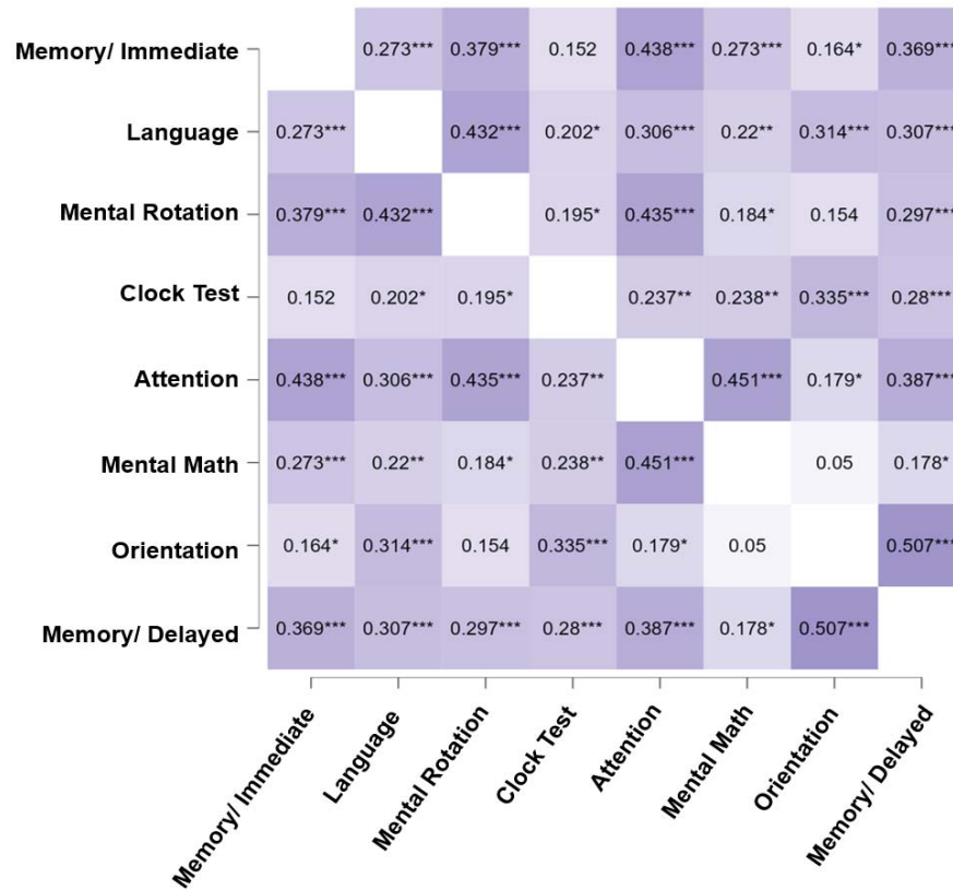
Figure 2- BOCA subscales correlation matrix. Heatmap representing significant Spearman correlations between BOCA subscales. Darker color represents a stronger relationship between variables. * = p<0.05 ; ** = p<0.01 ; *** = p<0.001 .
