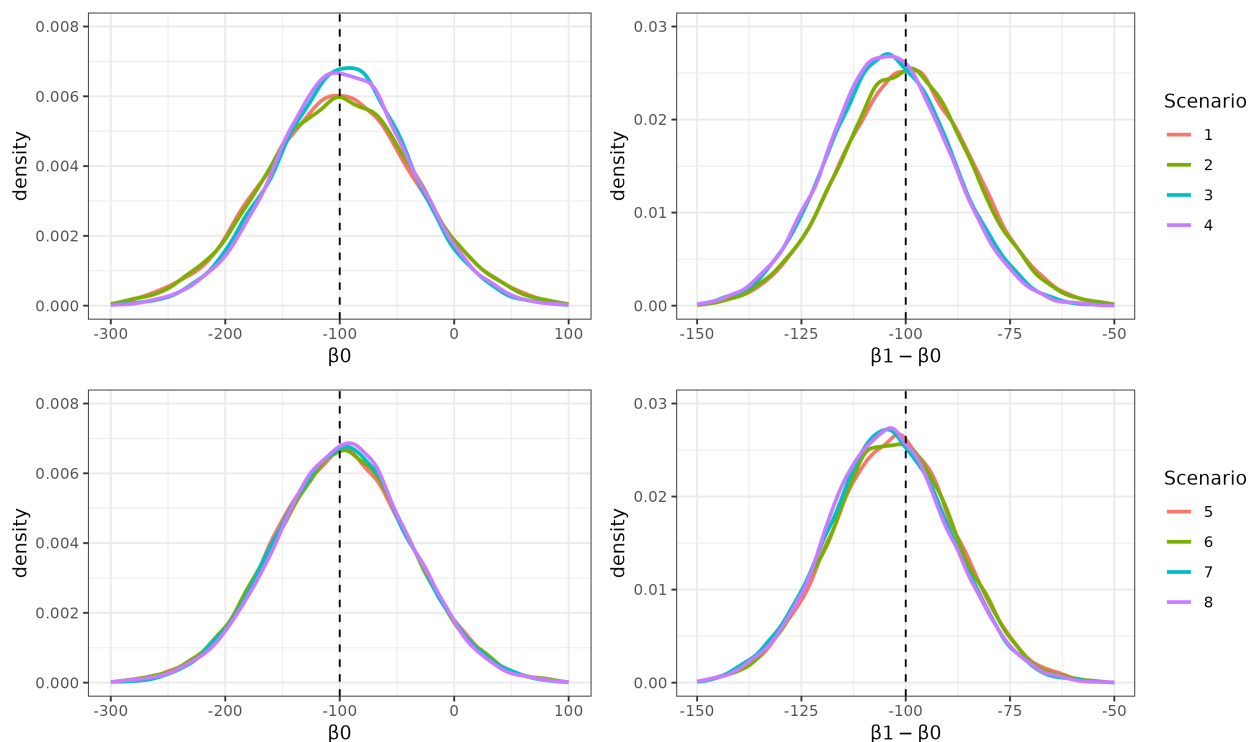
Figure 9: Density plots for the estimation of \beta_0 and \beta_1 - \beta_0 using method 2 over 20,000 simulation runs for 8 different scenarios.
