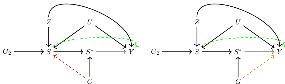
Figure 2: Left: DAG of linear interaction model from equation (1) highlighting in colour which assumptions need to hold for an unbiased estimate of \beta_1 and \beta_0 when using Method 1. Right: DAG of linear interaction model (1) highlighting in colour which assumptions need to hold for an unbiased estimate of \beta_1 and \beta_0 when using Method 2.
