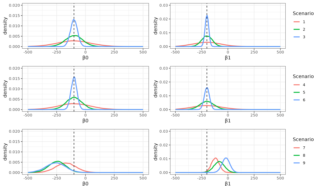
Figure 8: Density plots for the estimation of \beta_0 and \beta_1 using method 1 over 20,000 simulation runs for 9 different scenarios.
