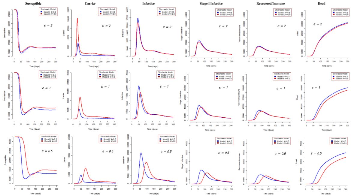
Fig. 6: Plots of the compartmental profiles for models I and II for \epsilon = 0.5, 1 and 2 for population size N = 5 \times 10^4
