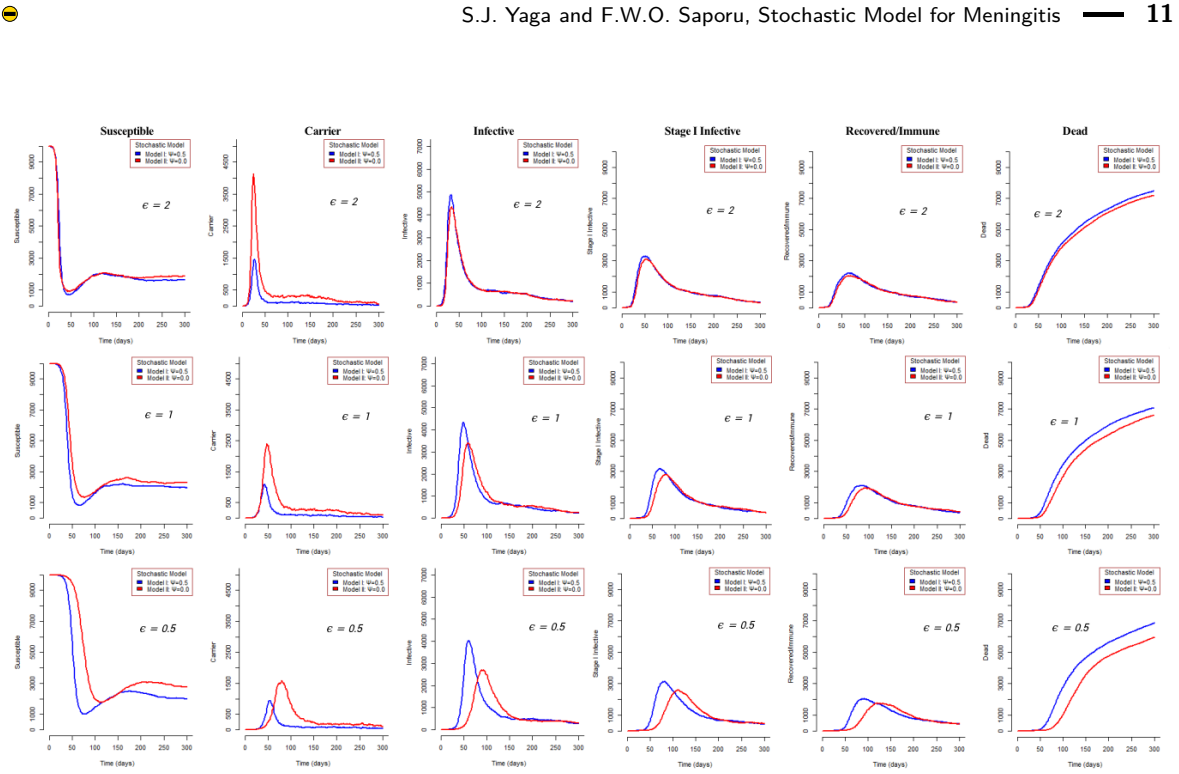
Fig. 5: Plots of the compartmental profiles for models I and II for \epsilon = 0.5, 1 and 2 for population size N = 10^4
