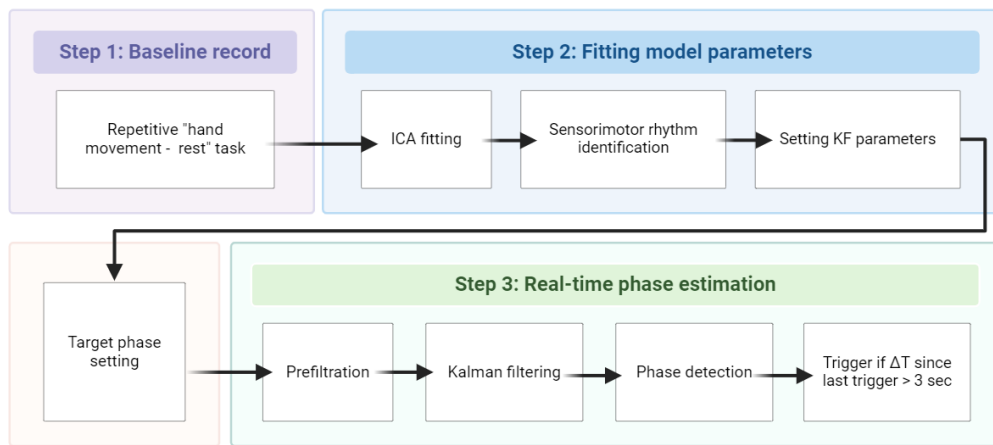
Figure 2. Computational pipeline
