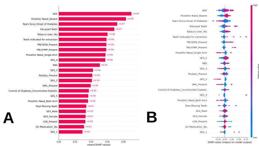
Fig. 2. SHapley Additive exPlanations plots: A- SHAP Bar Plot (Values represented are mean absolute SHAP values representing global feature importance); B- SHAP beeswarm plot (Individual dots represent the SHAP value of each data point, the colour of the dot denotes whether feature value was high or low)
