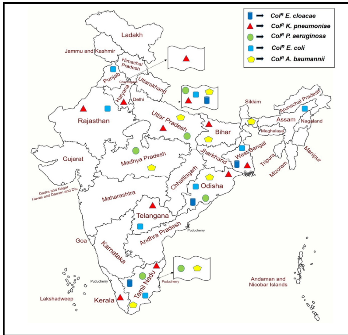
Figure 4. The reports of Col R GNB bacterial species from various states and Union Territories of India.
