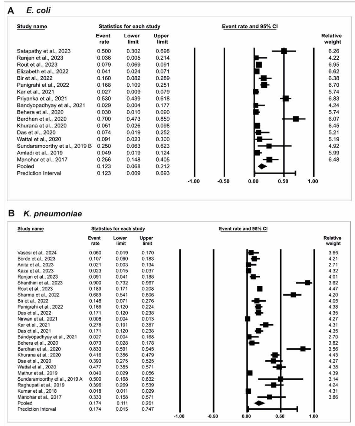
Figure 2. Forest plots demonstrating the pooled prevalence of Col R among (A) E. coli , and (B) K. pneumoniae . The Comprehensive meta-analysis software V4 (Biostat Inc. USA) was used for the calculation of the event rate, and 95% confidence interval, and used in the forest plot.
