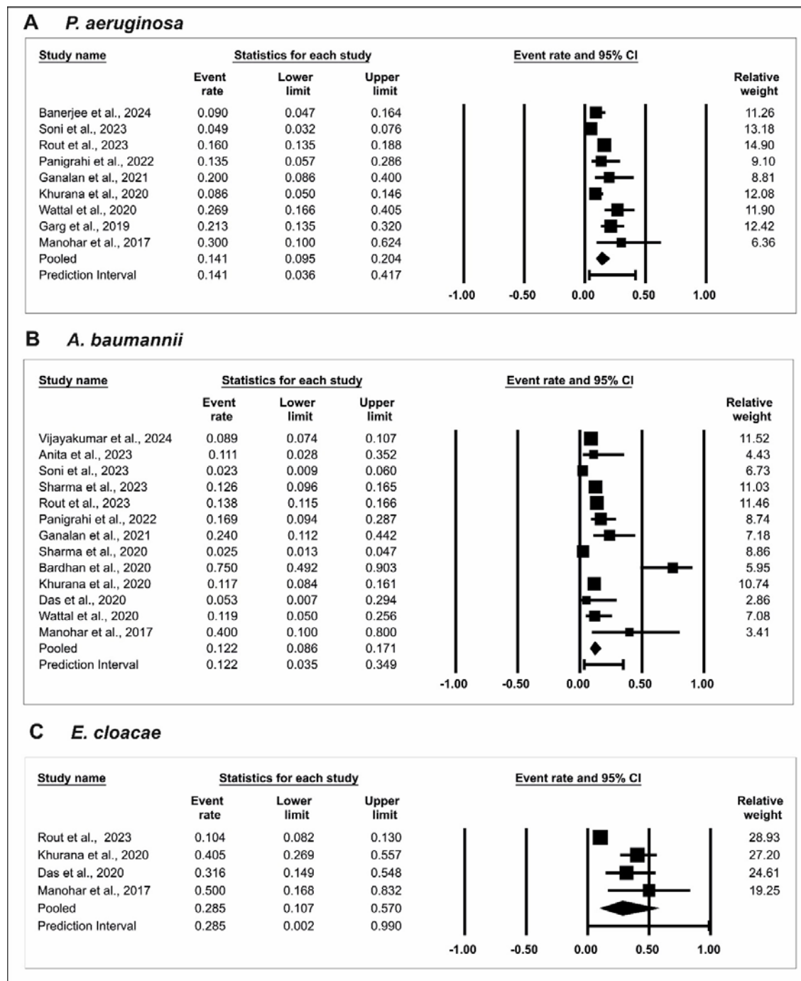
Figure 3. Forest plots demonstrating the pooled prevalence of Col R (A) P. aeruginosa , (B) A. baumannii , and (C) E. cloacae .
