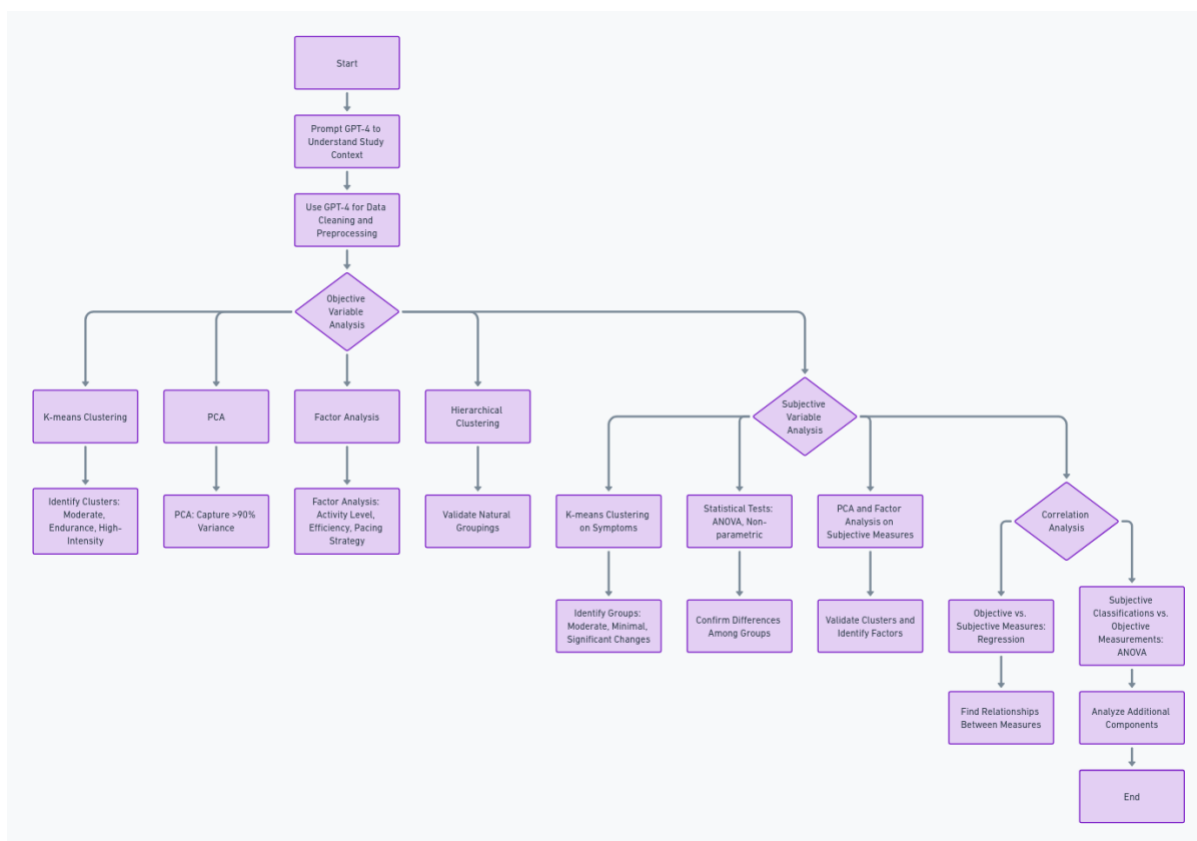
Figure 1. Schematic of statistical data analysis plan and its implementation via GPT-4
