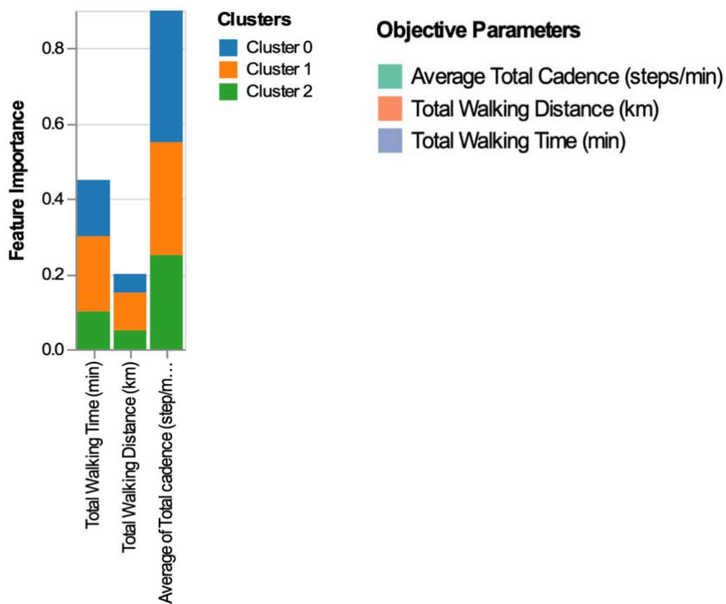
Figure 30. Feature Importance for Predicting Subjective Cluster Membership
