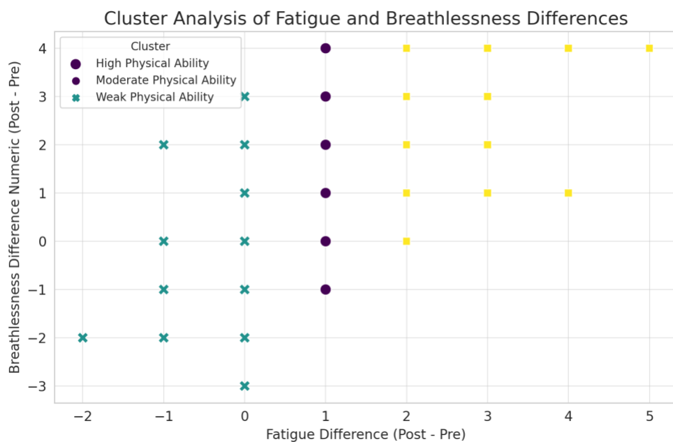
Figure 17: Scatter plot showing the clustering of physical ability based on differences in fatigue and breathlessness.
