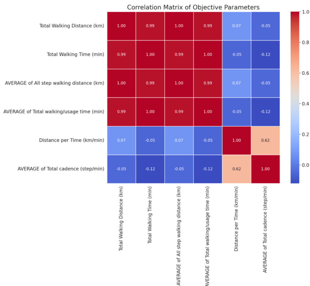
Figure 4. Heatmap illustrating the matrix of correlation coefficients among objective parameters during SIP exercise.
