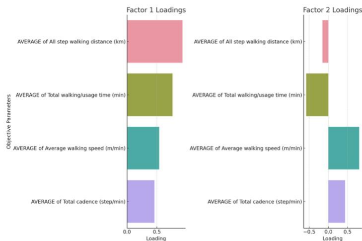
Figure 12. Factor loadings resulting from Factor Analysis on the objective parameters.
