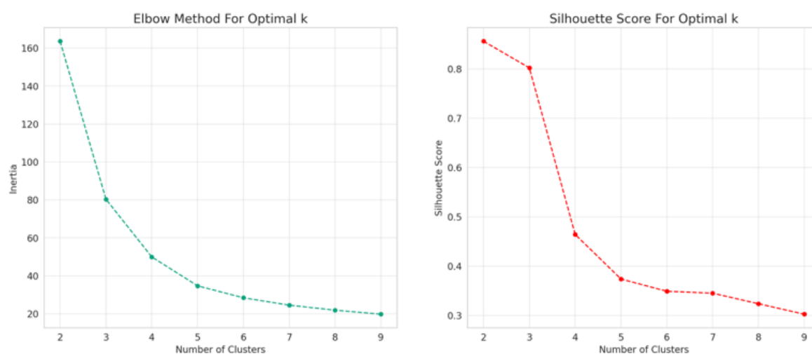
Figure 6. Elbow Method for determining the optimal number of clusters in K-means clustering analysis of objective parameters. Silhouette Score analysis for determining the optimal number of clusters in K-means clustering analysis of objective parameters.
