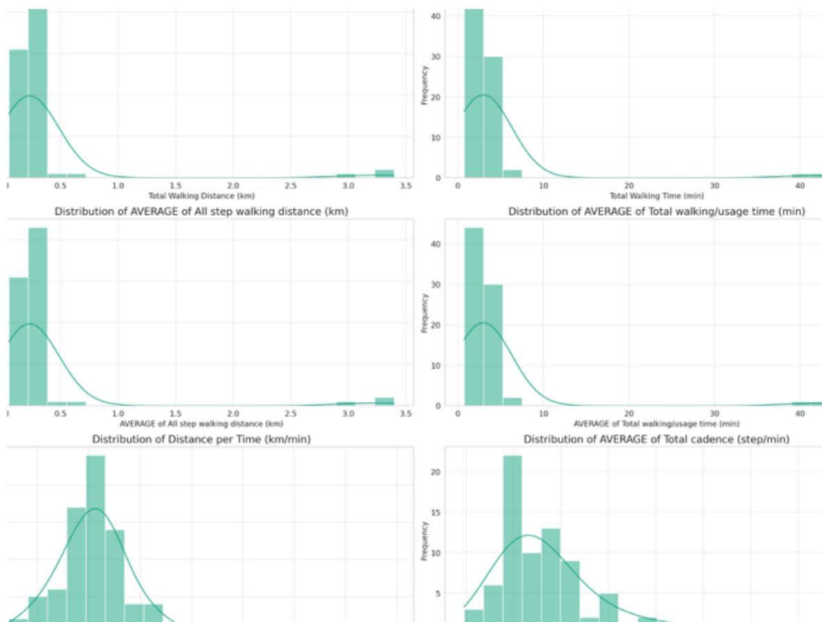
Figure 2. Histograms illustrating the distribution of objective parameters from the SIP exercise data.
