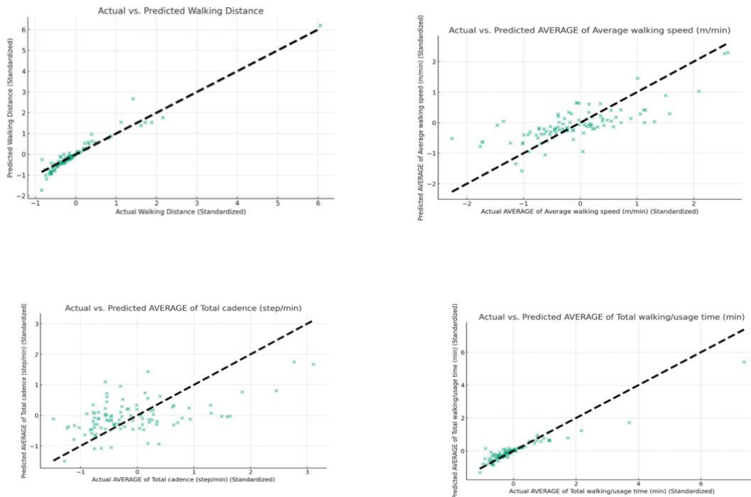
Figure 3. Predicted versus actual plot illustrating the parametric predictability of the regression model described in the text.
