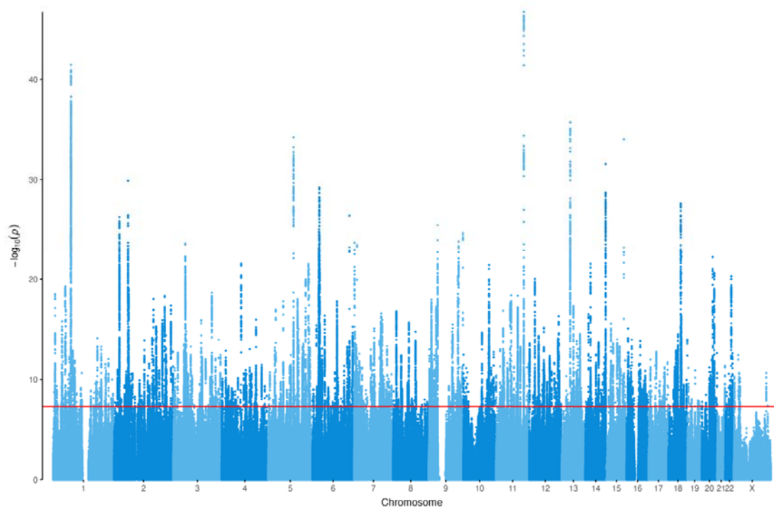
Figure 1: Manhattan Plot of GWAS meta-analysis of 685,808 MD cases and 4,364,225 controls
