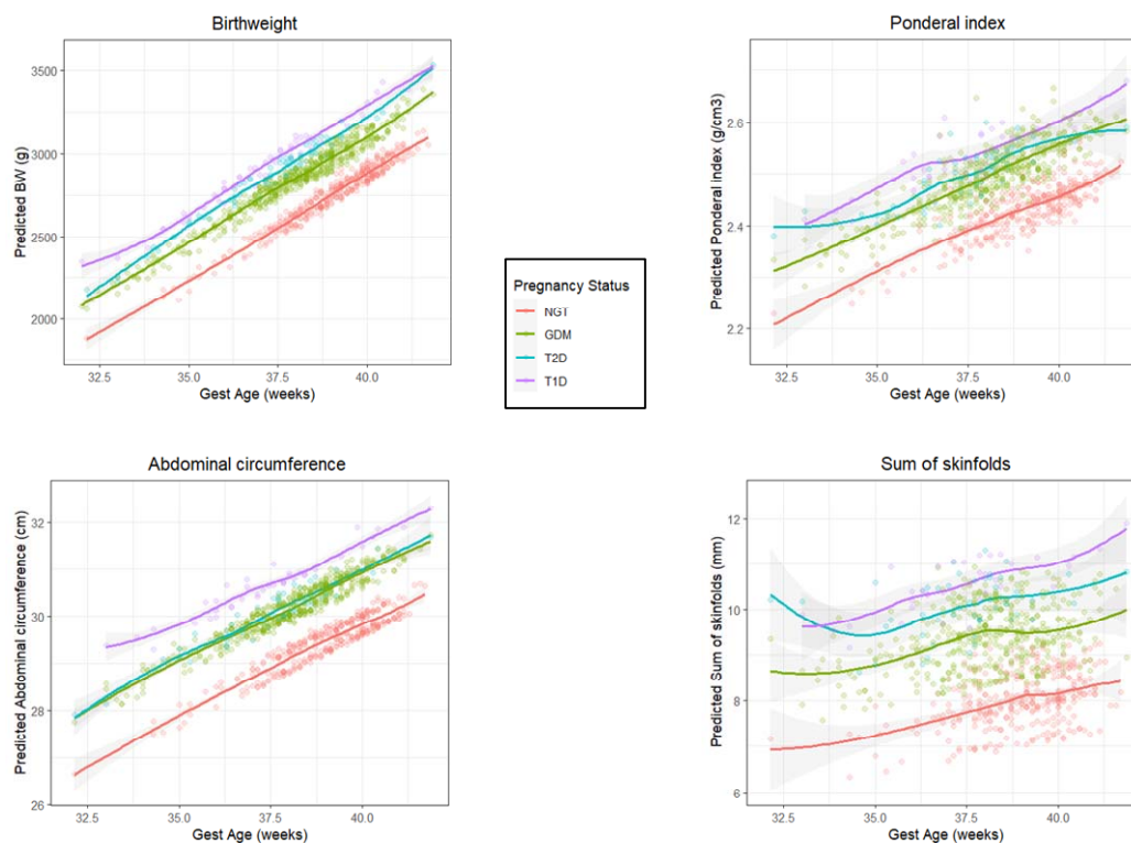
Figure 2 Prediction curves for obesity-adiposity measurements in neonates born to mothers with diabetes (type 1, type 2 and GDM) or NGT between gestational age 32 and 42 weeks
