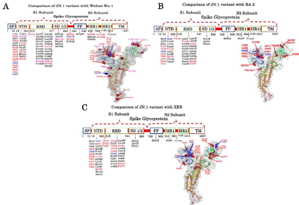
548 549 FIGURE 2 Amino acid changes in the different domains of JN.1 in comparison with Wuhan- 550 Hu-1 , BA.2, and XBB (Red colour indicates the unique mutations, the blue colour indicates 551 the dynamic mutations, the black colour indicates random mutations and pale red indicates 552 universal mutations). Fusion peptide (FP), Heptad Repeat (HR1/2), N-terminal domain (NTD), 553 Receptor Binding Domain (RBD), Signal peptide (SP), Spike Subdomain (SD) and 554 Transmembrane domain (TM) are the different motifs of the spike glycoprotein.
