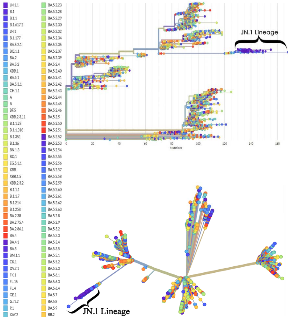
558 FIGURE 3 The phylogenetic analysis of the JN.1 variant using a rooted tree and an unrooted 559 tree illustrates the evolutionary relatedness among the sequences of JN.1 (n=66) compared 560 with the reference genome of SARS-CoV-2 ( Wuhan-Hu-1 ).
