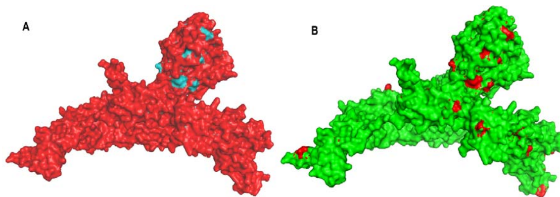
FIGURE 4 Superimposition of protein models. A: Superimposed protein model of Wuhan Hu-1 reference model (red) with JN.1 specific mutations (blue). B: Superimposed protein model of JN.1 variant (green) with the study-specific unique mutation model identified in our study patients (red).
