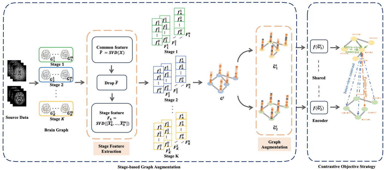
Fig. 1. The overview of SF-GCL.
