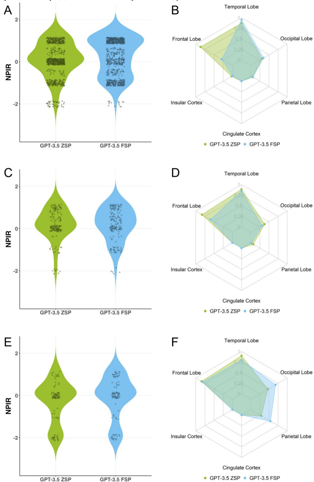
Figure 1: (A) Net Positive Inference Rate (NPIR) distribution for GPT-3.5 with zero-shot prompting (ZSP) and few-shot prompting (FSP) on the public-source database. (B) Regional sensitivity (RSens) for GPT-3.5 ZSP and FSP on the public-source database. (C) NPIR distribution on the private-source database. (D) RSens on the private-source database. (E) NPIR distribution on the 100-question survey. (F) RSens on the 100-question survey.
