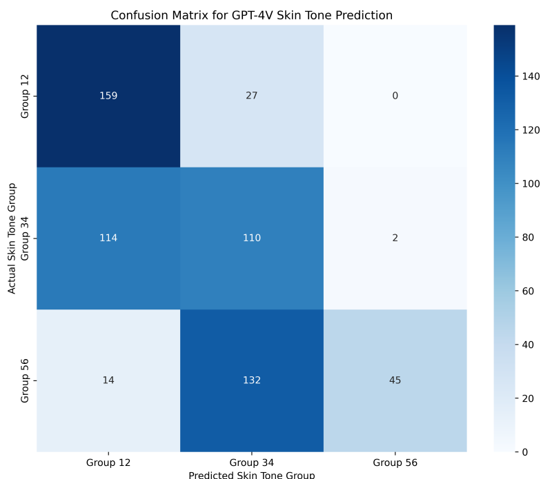
Fig. 2 This shows the confusion matrix for the Fitzpatrick skin tone (FST) prediction. We see that GPT-4V misses many of the darker skin tones and performs worse in this group.
