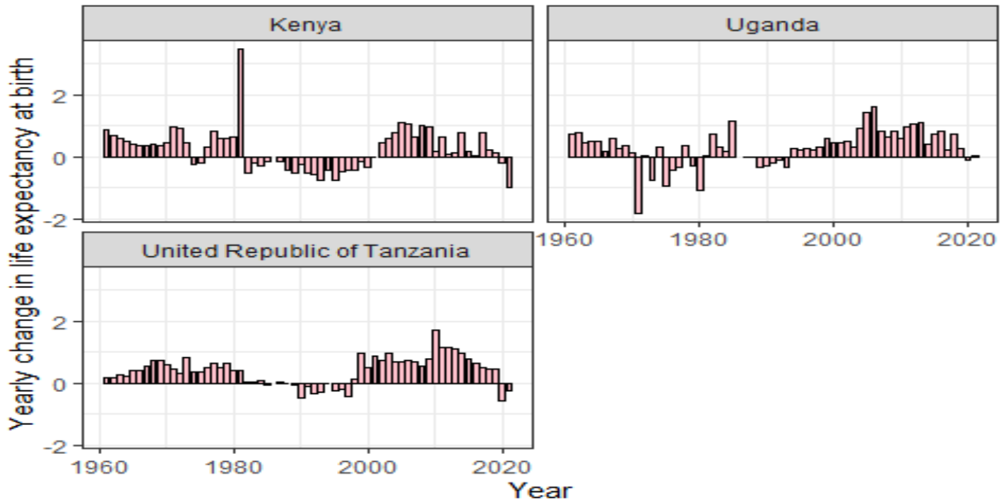
Figure 4: Life expectancy changes among females in Kenya, Uganda, and The United Republic over 61 years (1960-2021). The figure shows that in Kenya, life expectancy gains among females were observed between 1960 to 1973, then 1975 to 1982, however, losses were observed between 1974-1975; 1982-2000; and 2020-2021. In Uganda, life expectancy gains in females were between 1960-1970 but losses were observed between 1971-1981 and between 1988-1993, and in 2020. In the United Republic of Tanzania, life expectancy gains among females were observed between 1960-1985 but losses were observed between 1986-1997 and 2020-2021.
