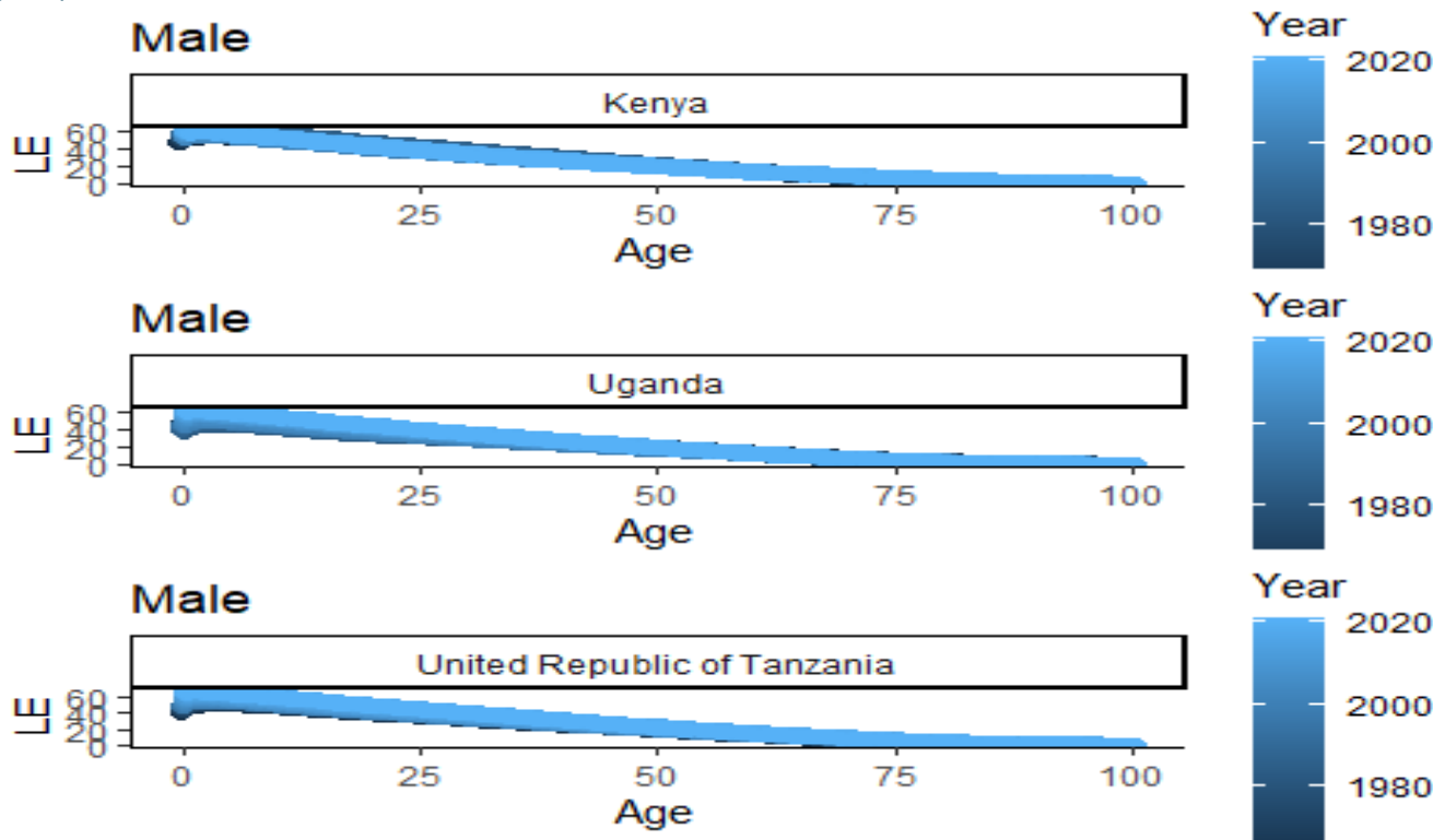
Figure 1: Life expectancy variations by years in Kenya, Uganda, and the United Republic of Tanzania over 61 years (1960-2021). These graphs show visual variations in the evolution of life expectancy over the years for different age groups in Kenya, Uganda, and the United Republic of Tanzania. From these graphs, it is evident that LE_0 in Tanzania and Uganda have gradually increased over the years across all age groups. Also, in Kenya, life expectancy at age 0 and 60 and above have shown gradual increases over the years. However, for ages 1 to 59, it is noticeable that life expectancy was higher from 1969 to 1992, whereas in recent years, there has been a decline in life expectancy in this age group. This decline is observed in males and females.
