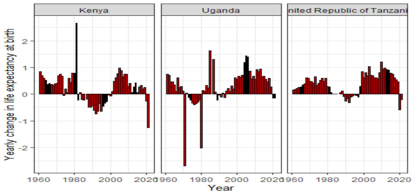
Figure 3: Life expectancy changes in Kenya, Uganda, and United Republic over 61 years (1960-2021). The figure shows that in Kenya, life expectancy gains were observed between 1960 to 1981 however, losses were observed between 1982 to 2000 and also 2020 to 2021. In Uganda, life expectancy gains were observed between 1960 to 1970 and losses were observed between 1971 to 1980 and also between 2020 to 2021. In the United Republic of Tanzania, life expectancy gains were observed between 1960 to 1985 but losses were observed between 1989 to 1998 and 2020 to 2021.
