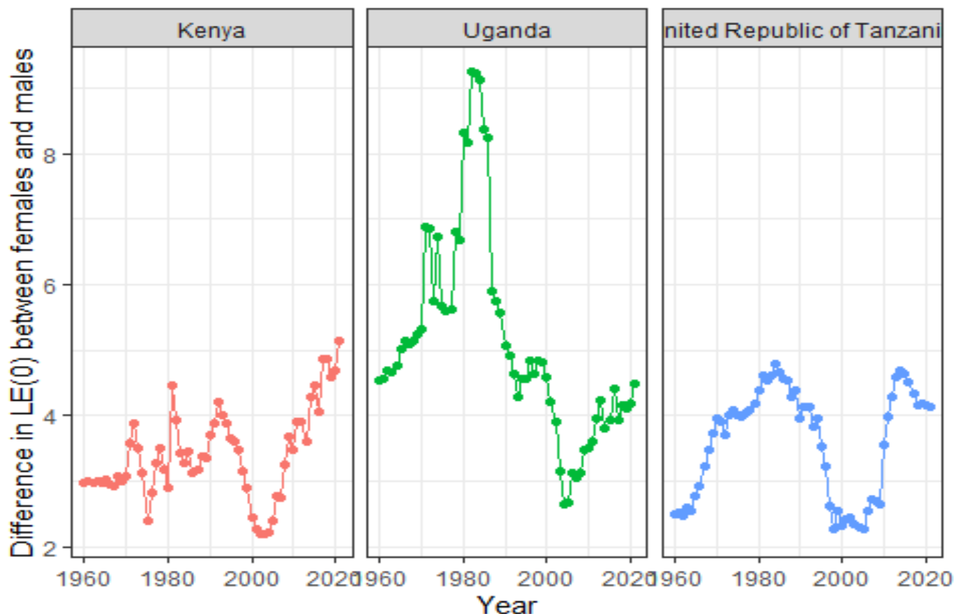
Figure 6: Gaps in life expectancy between males and females in Kenya, Uganda, and The United Republic of Tanzania over 61 years (1960-2021).
