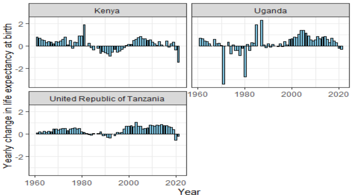
Figure 5: Life expectancy changes among males in Kenya, Uganda, and The United Republic over 61 years (1960-2021). The figure shows that in Kenya, life expectancy gains among males
