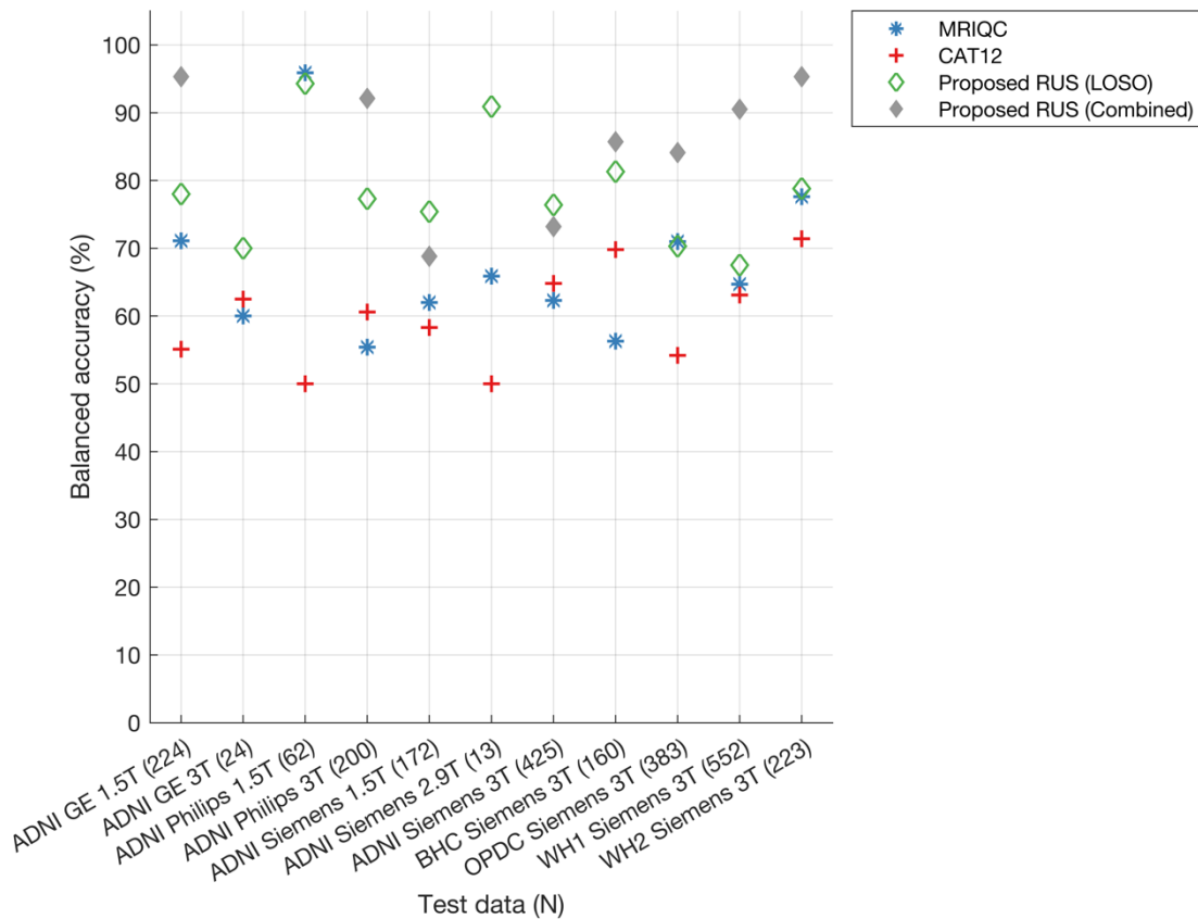
Figure 10. Balanced accuracy of MRIQC, CAT12 and the proposed RUS classifier. The total number of samples for each test site are provided in brackets (x-axis). For RUS classifier, each site was kept as test data and classifier was trained on remaining sites using the hyperparameters and feature ranking derived from combined data model (best model with 80 Feature size). For reference, we also provide the balanced accuracy of RUS classifier for each site within the test data of the combined data model to see how well our classifier generalises to test data from different sites (diamond marker with grey colour). Note that balanced accuracies for the combined data model are not included for three sites (ADNI GE 3T, ADNI Philips 1.5T and ADNI Siemens 2.9T) due to the absence of samples in the reject class of the test data (resulting in NaN values for balanced accuracies)
