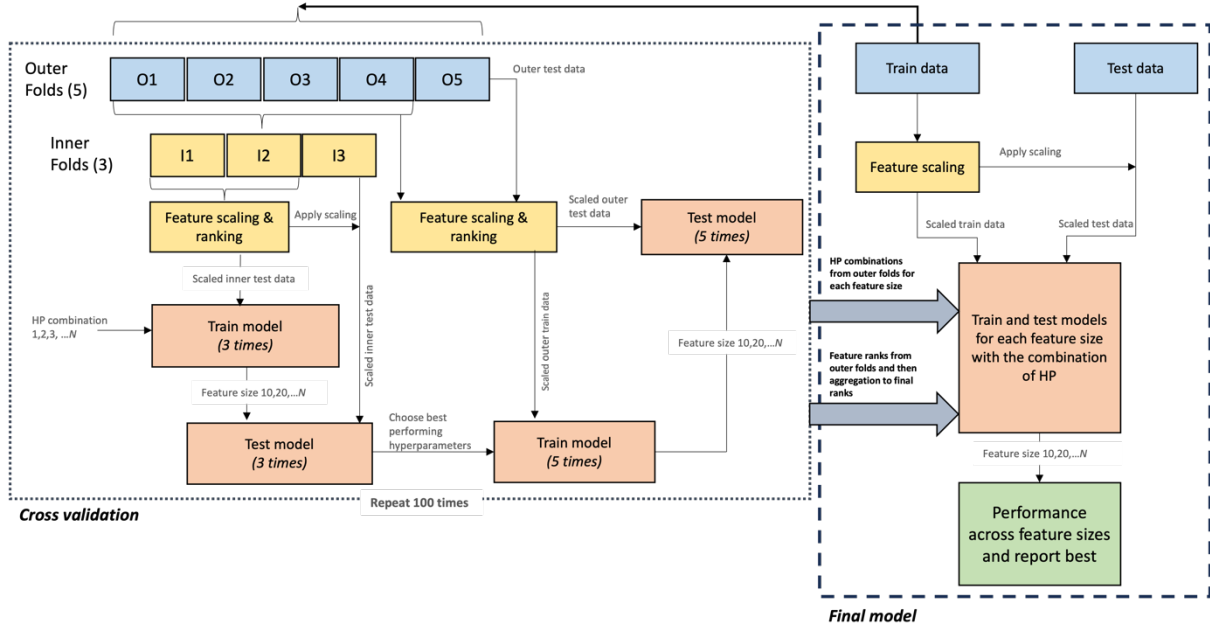
Figure 1. Nested cross validation workflow for training the QC classifier. The model was trained for 5 outer folds and 3 inner folds. The hyperparameters of the model were optimised on the inner test data and the combination giving the best performance (balanced accuracy) were selected for the outer folds. The nested cross validation process was repeated for 100 times. The best performing hyperparameters for each feature size and feature ranks across 100 iterations were used to train the final model and tested on the hold-out data.
