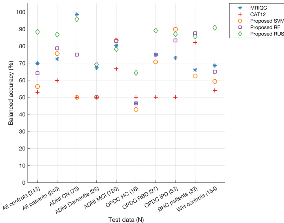
Figure 6. Balanced accuracy of proposed classifiers, MRIQC, and CAT12 analysed separately for scans from healthy individuals, patients, and each diagnostic sub-category within both healthy and patient groups in the test dataset. Number of samples in the test data are provided in brackets for each category (x-axis). Legend of diagnostic subgroups: CN = cognitively normal; HC = Healthy Controls; MCI = Mild Cognitive Impairment; RBD = REM Sleep Behaviour Disorder; iPD = idiopathic Parkinson’s Disease.
