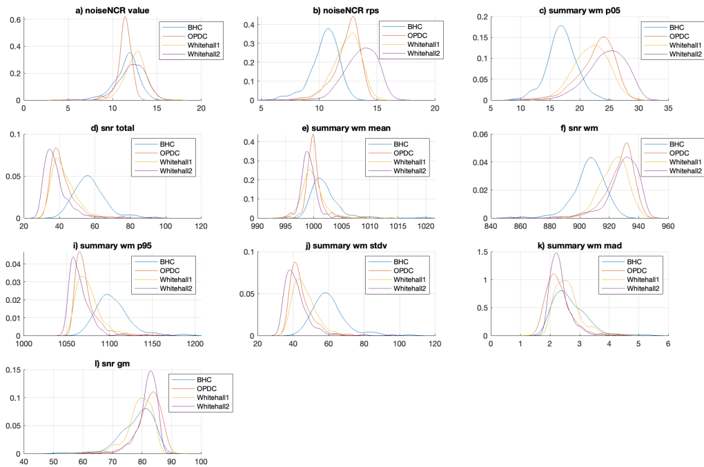
Figure 8. Kernel density plots showing the distribution of top 10 ranked features in final combined data model for BHC, OPDC, Whitehall1 and Whitehall2 sites. For a description of the features, please refer to tables Table 2 and Table 3 .
