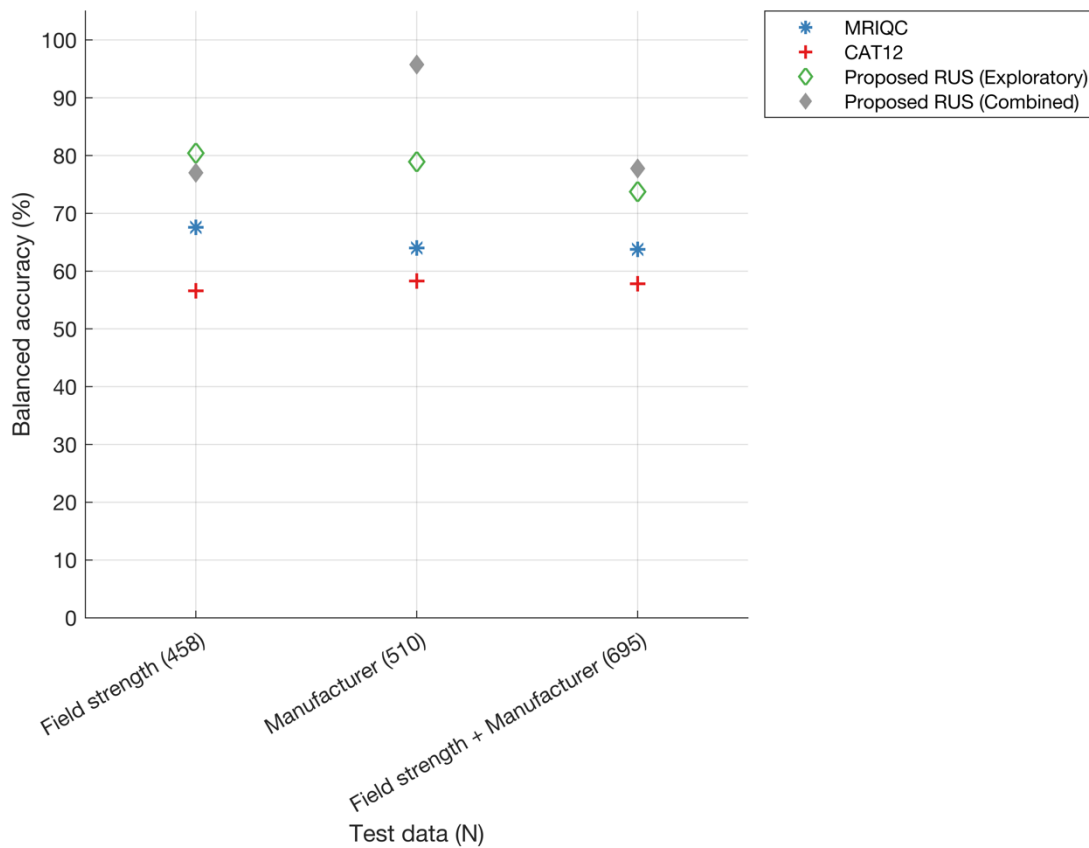
Figure 11. Balanced accuracy of MRIQC, CAT12 and the proposed RUS classifier for exploratory models. The total number of samples for each test site are provided in brackets (x-axis). Field strength: performance of models trained on 3T scanners data (Siemens, Philips, GE) and tested on 1.5T (Siemens, Philips, GE) and 2.9T (Siemens) scanners data; Manufacturer: performance of models trained on Siemens (1.5T, 2.9T, 3T) data and tested on Philips (1.5T, 3T) and GE (1.5T, 3T) data; Manufacturer and field strength: performance of models trained on Siemens 3T data and tested on Siemens (1.5T, 2.9T), Philips (1.5T, 3T) and GE (1.5T, 3T) data. Additionally, the balanced accuracy of the RUS classifier within the test data for the combined data model for each scenario is presented for reference (diamond marker with grey colour).
