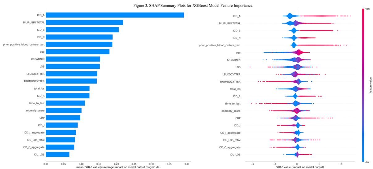
381 382 383 Figure 3. SHAP Summary Plots for XGBoost Model Feature Importance. Bar plot on the left illustrating the global feature importance 384 ranked by the sum of SHAP values across all samples. On the right is the Beeswarm plot detailing the individual SHAP values for each 385 feature and their impact on the model's output.
