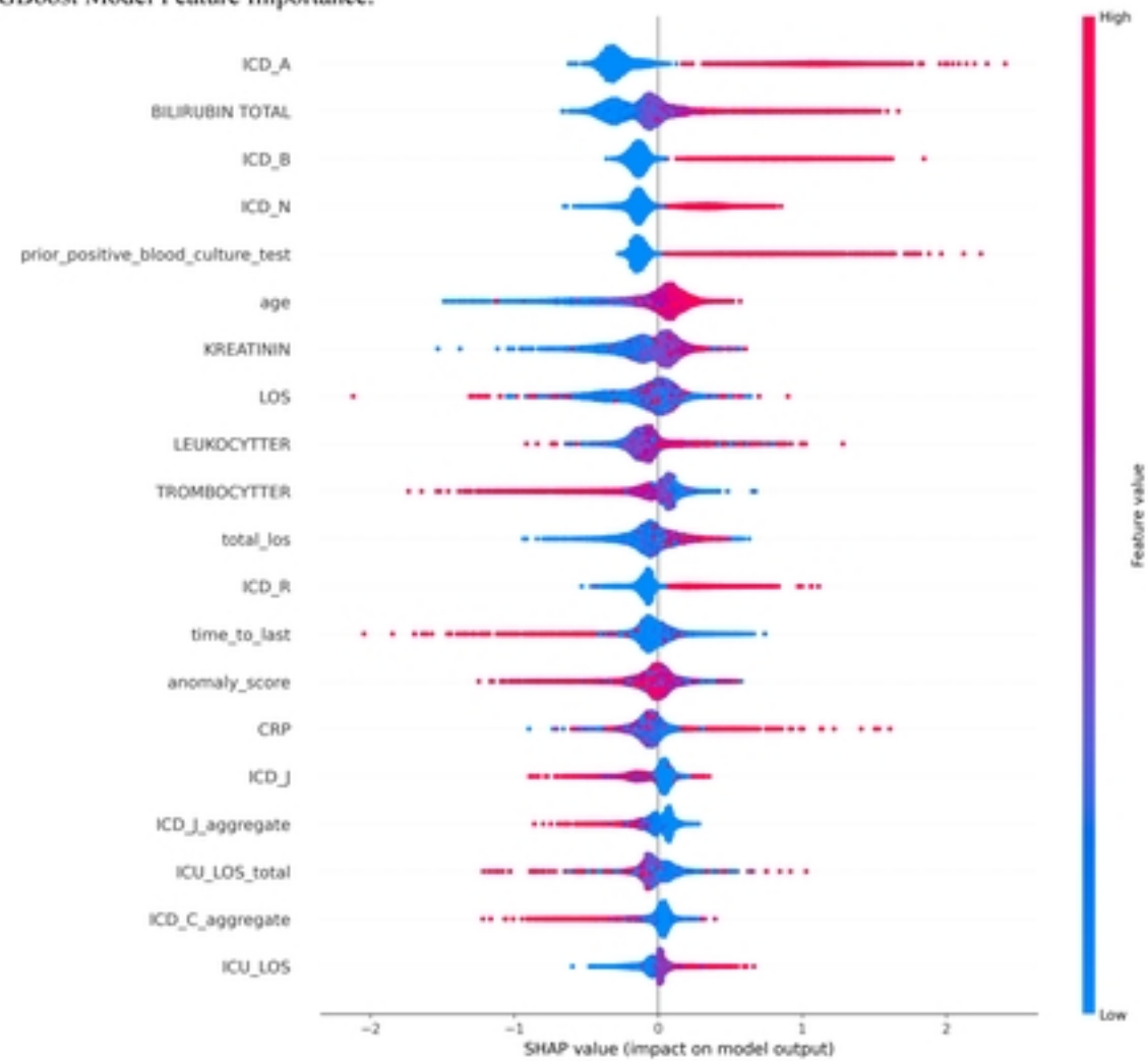
Figure 3. SHAP Summary Plots for XGBoost Model Feature Importance.
