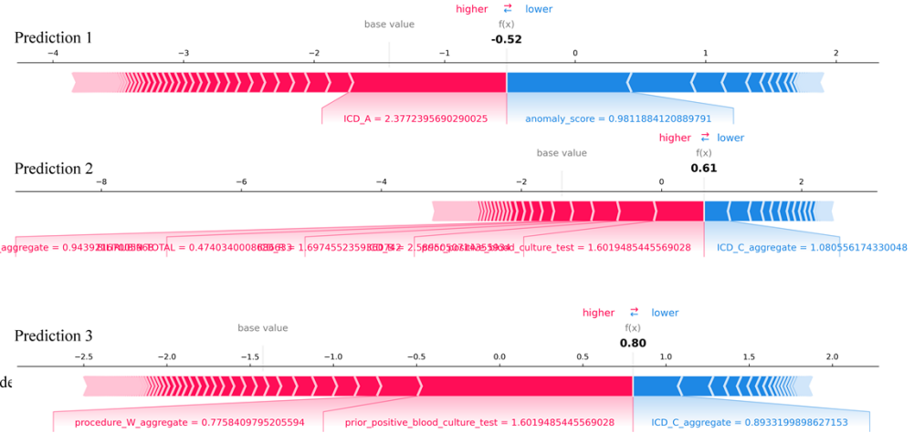
Figure 4. Waterfall and Force plots of first three predictions from the testing set.
