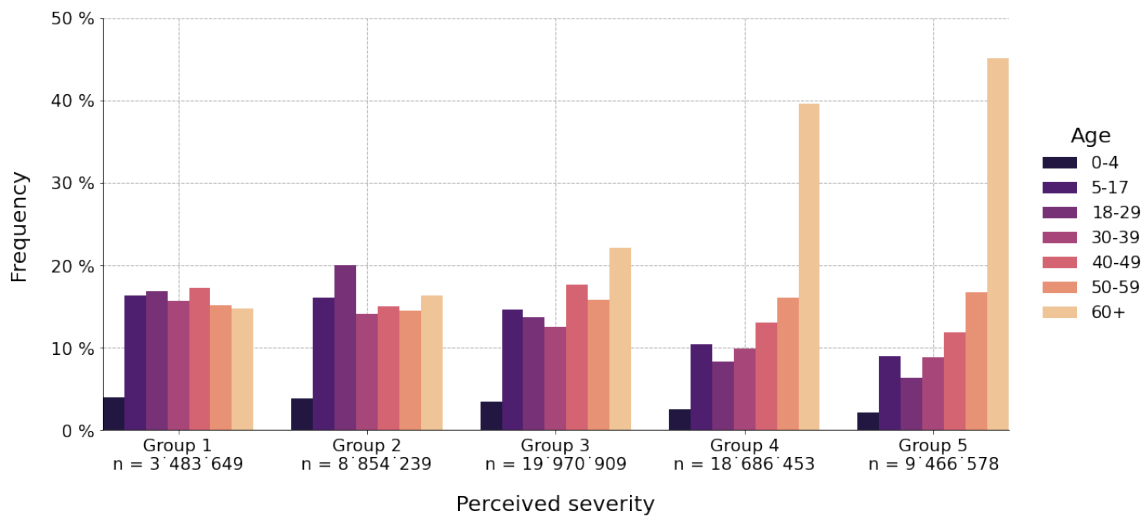
Figure 4: Distribution of age in each perceived severity group. We also report the total number of individuals in each group.
