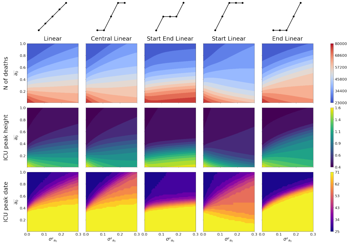
Figure 6: Heatmaps showing the number of deaths (first row), the height of the ICU peak (second row) and its date (third row) as a function of \bar{a}_0 and \sigma^2_{a_0} . Each column corresponds to one of the five functions linking perceived severity and midpoint of the logistic curve giving the transition rate from compliant to non-compliant compartments as a function of the fraction of vaccinated individuals. Above each column is a small diagram of the function, showing how the midpoint a_0 varies, going from small to high perceived severity groups (left to right). The other parameters used for the simulations are \alpha = 10 , \gamma = 5 , \bar{b}_0 = 0.75 , \sigma^2_{b_0} = 0 . We employed a 900-value grid, with 30 values of \bar{a}_0 ranging from 0 to 1, and 30 values of \sigma^2_{a_0} ranging from 0 to 0.3. The rugged profile of the curves related to the peak date is due to its discrete nature, with values representing the (integer) number of days after the simulation's start in which the peak is observed.
