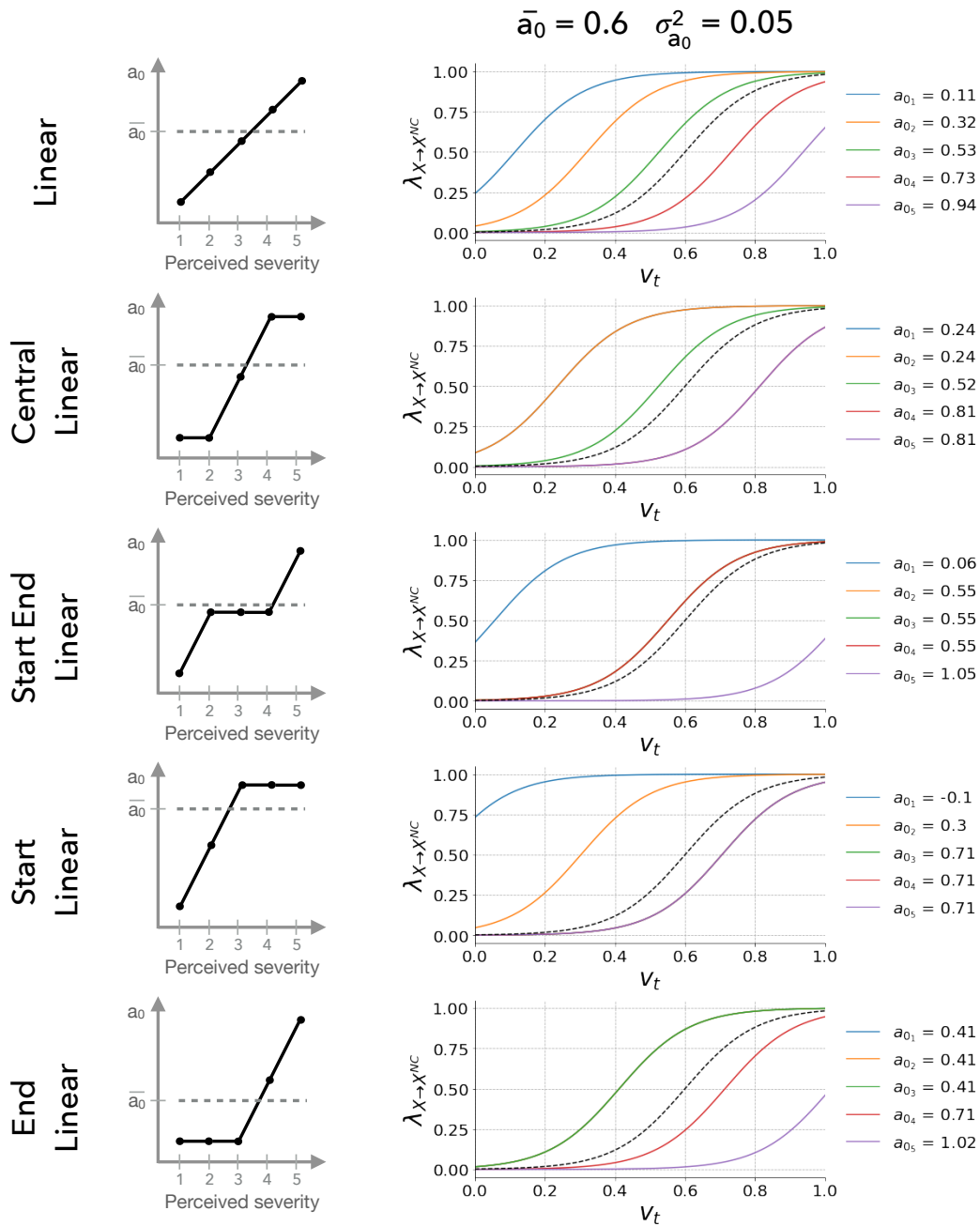
Figure 3: Left column: Sketch of the 5 functions used to model the dependency of the midpoint from perceived severity. From top to bottom, Linear, Central Linear, Start End Linear, Start Linear, End Linear. The horizontal dashed lines give the average \bar{a}_0 = 0.6 . Right column: logistic curves as a function of the fraction of vaccinated individuals, for the various midpoints obtained with a fixed average \bar{a}_0 = 0.6 and either variance 0 (dashed line, in which case all midpoints are equal to the average) or variance \sigma_{a_0}^2 = 0.05 .
