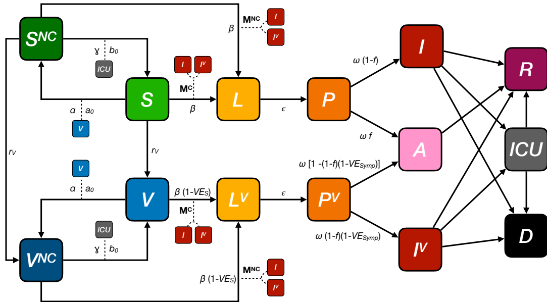
Figure 1: Model diagram. The model is an extension of a standard SLIR (Susceptible-Latent-Infected-Recovered) with the addition of individuals who are pre-symptomatic ( P ) and asymptomatic ( A ) and also individuals in Intensive Care Units ( ICU ), and individuals who die ( D ). Furthermore, we introduced an additional series of compartments for vaccinated individuals ( V , L^V , P^V , I^V ) and two compartments ( S^{NC} and V^{NC} ) for individuals that relax their protective behaviors. Those individuals have a higher risk of infection, modeled using a contact matrix M^{NC} with a greater number of contacts than the one used for compliant compartments ( S and V ), M^C . Both matrices M^C and M^{NC} capture contact patterns of the winter period 2020-2021 in Italy, for regions with, respectively, high and small stringent restrictions.
