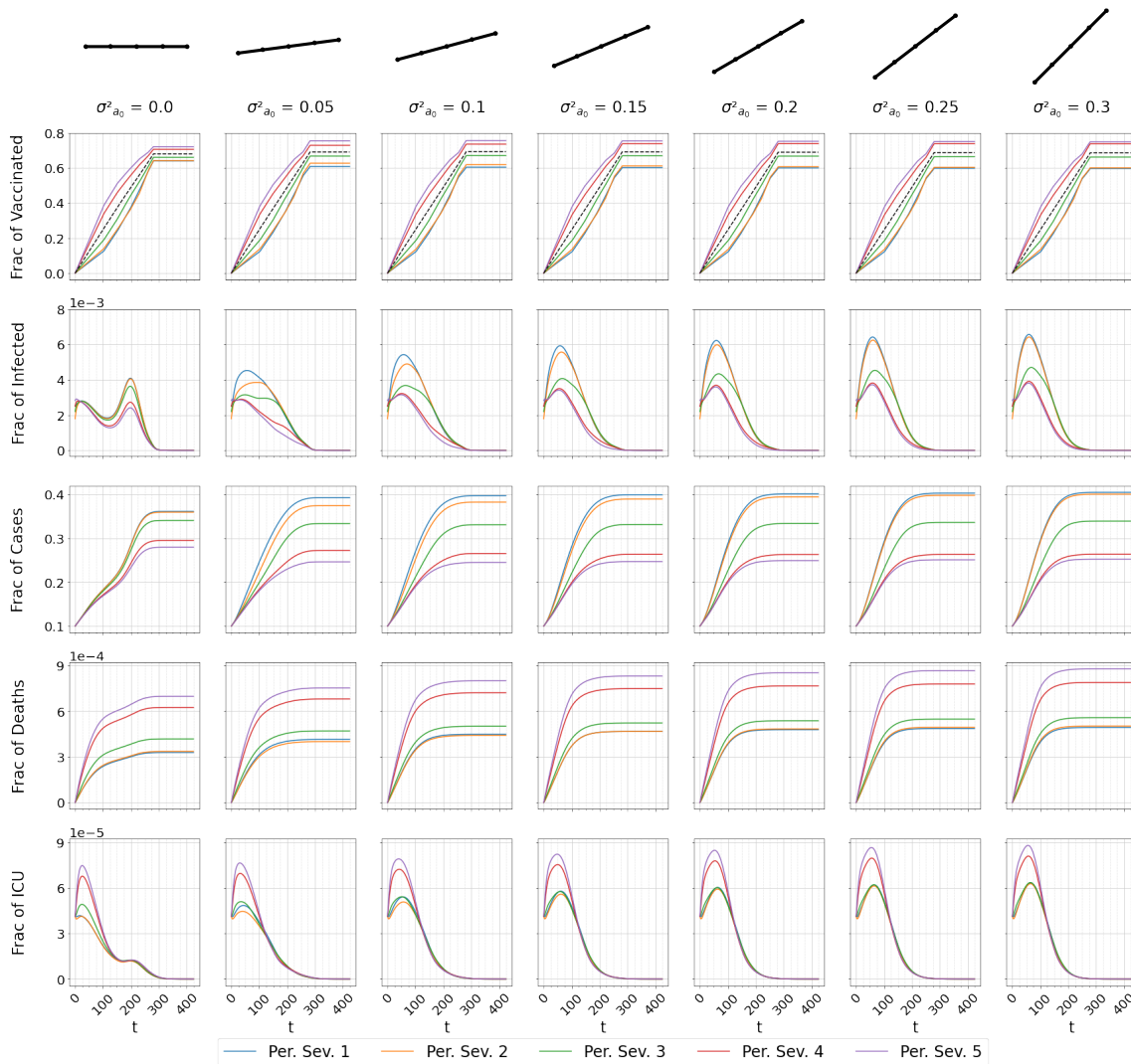
Figure 7: Fraction of vaccinated individuals (first row - the black dashed line reports the global fraction of vaccinated individuals in the population), infected individuals (second row), cases (third row - obtained as the sum of recovered individuals and deaths), deaths (fourth row), and individuals in ICU (fifth row) as a function of time (days), for each perceived severity group. Each column corresponds to a different value of the variance \sigma^2_{a_0} , going from 0 to 0.3, with \bar{a}_0 = 0.6 . The other parameters are \alpha = 10 , \gamma = 5 , \bar{b}_0 = 0.75 , and \sigma^2_{b_0} = 0 .
