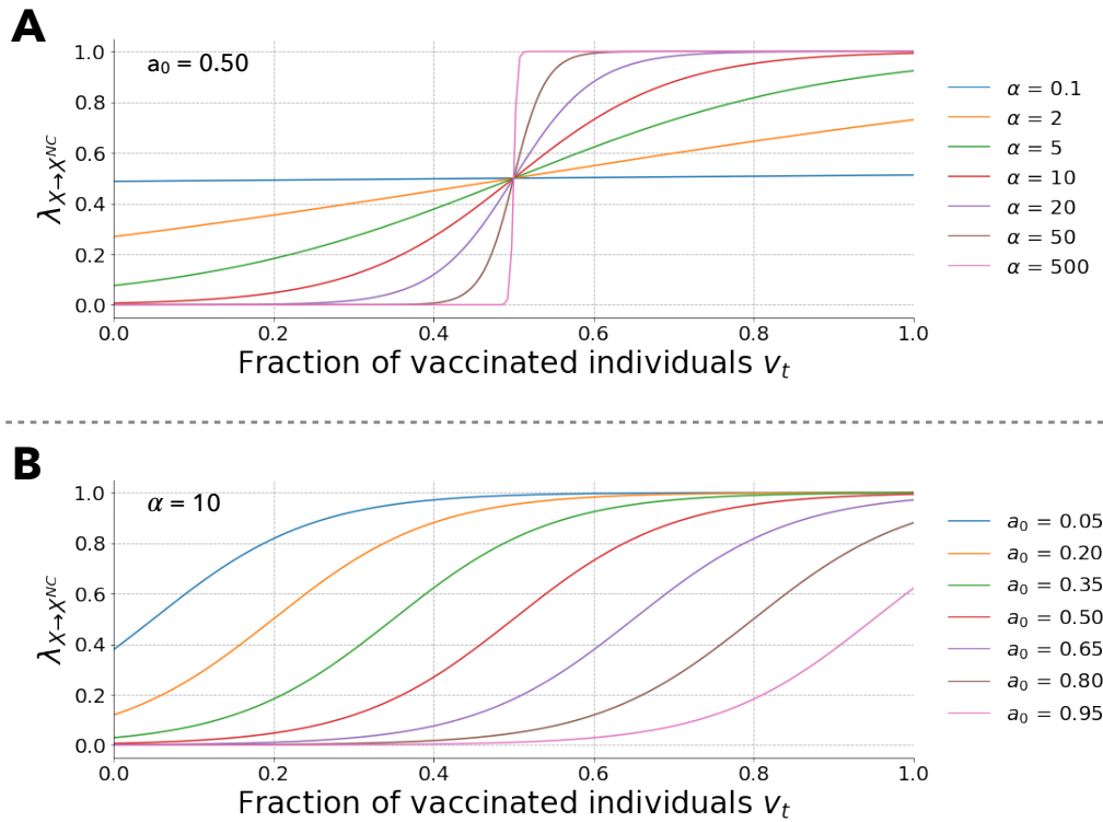
Figure 2: Rate of transition from compliant to non-compliant compartments as a function of the fraction of vaccinated population for several values of A) the slope \alpha with a fixed midpoint of a_0 = 0.5 , and B) the midpoint a_0 with a fixed slope of \alpha = 10 .
