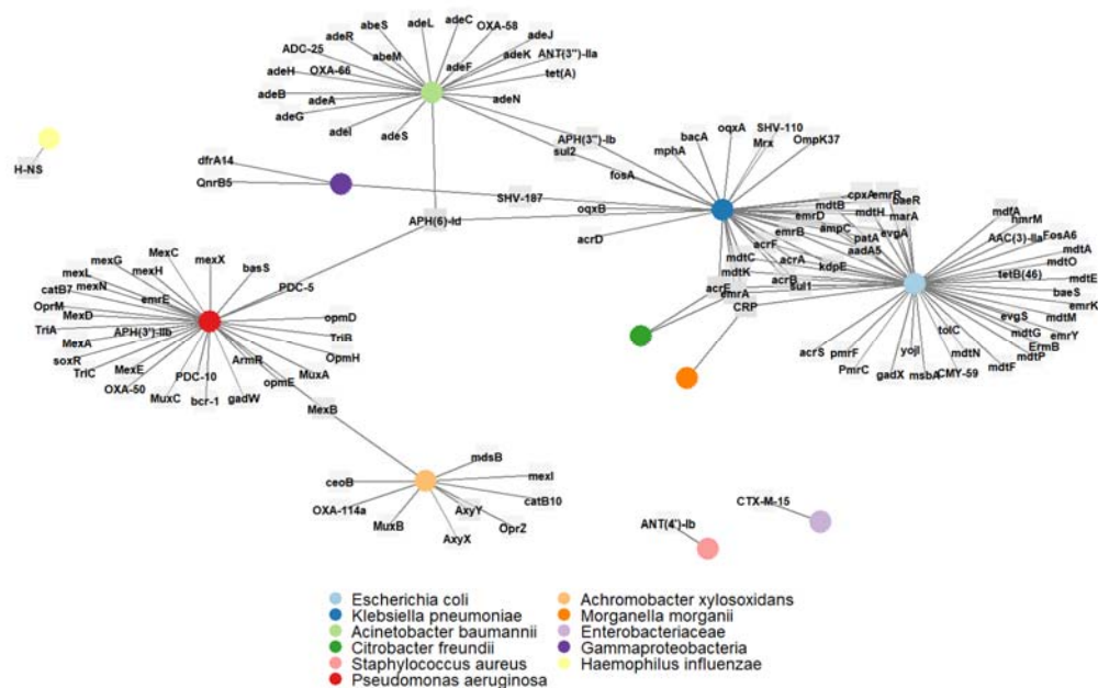
Figure 2. Network depicting the relationships between the AMR resistances and the bacterial taxonomy based on the contigs assembled in the AMR-positive patients.
