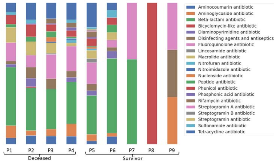
Figure 1. (Upper panel) Absence-presence matrix for AMR resistance groups identified among the nine AMR-positive patients. Numbers in boxes denote the number of different ARGs identified per patient. (Lower panel) Relative abundance of resistances as classified in resistance groups in the nine AMR-positive patients.
