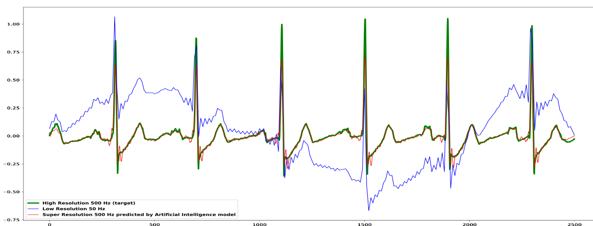
Figure 2: Input: LR corrupted signal sampled at 50 Hz (blue), Target: HR clean signal sampled at 500 Hz (green), Output: predicted SR denoised signal sampled at 500 Hz. Lead I only reported for simplicity.
