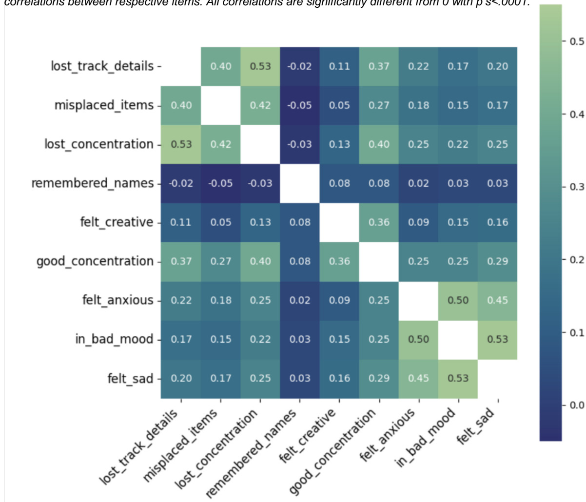
Figure 1. Inter-item correlation coefficients of original nine-item survey in Experiment 1. Warmer colors show stronger correlations between respective items. All correlations are significantly different from 0 with p 's<.0001.
