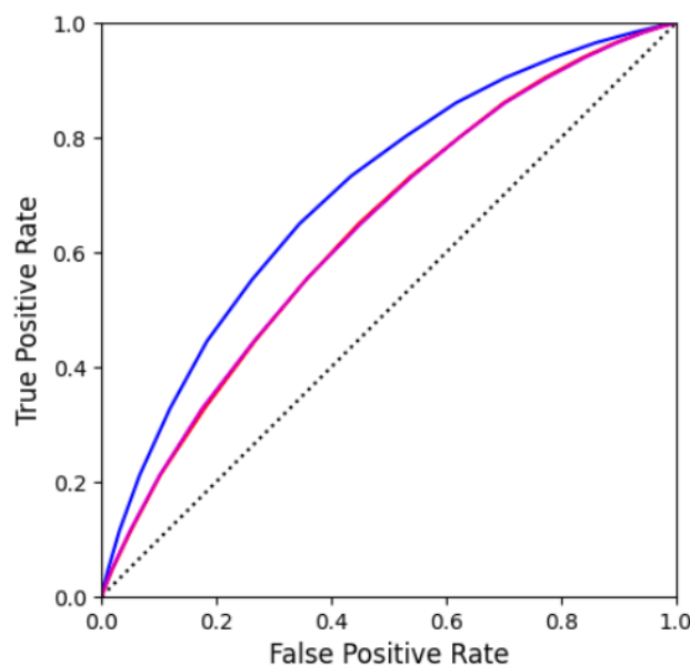
Figure 4A. Known-groups validity with ROC curves of BAMS-7 Attention subscale in ADHD, Anxiety, and Depression cohorts in Experiment 3.
