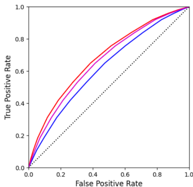
Figure 4B. Known-groups validity with ROC curves of BAMS-7 Mood subscale in ADHD, Anxiety, and Depression cohorts in Experiment 3.
