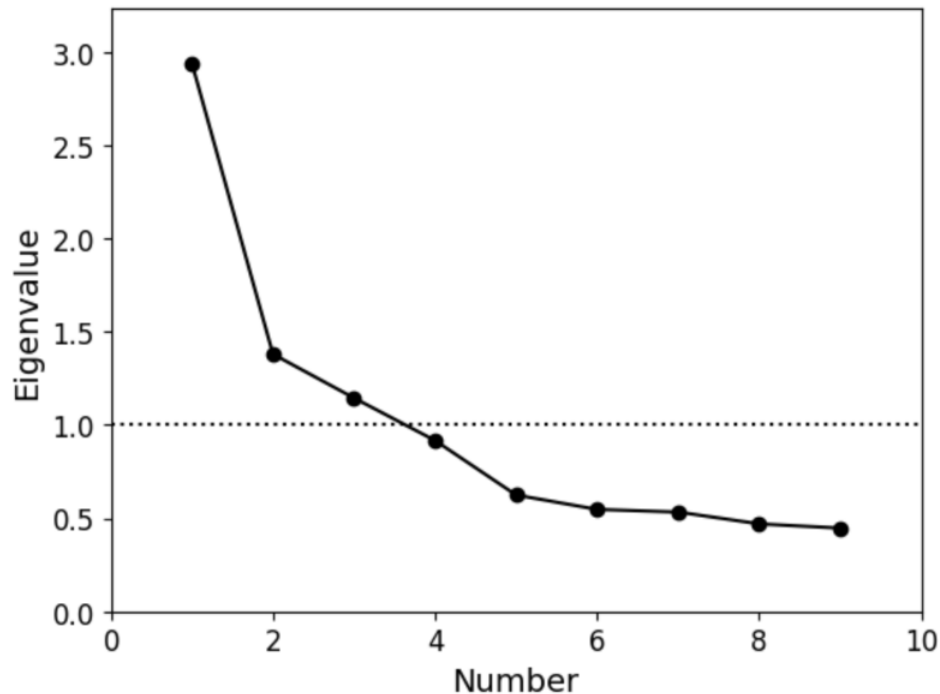
Figure 2. Scree plot for exploratory factor analysis of original nine-item survey in Experiment 1.
