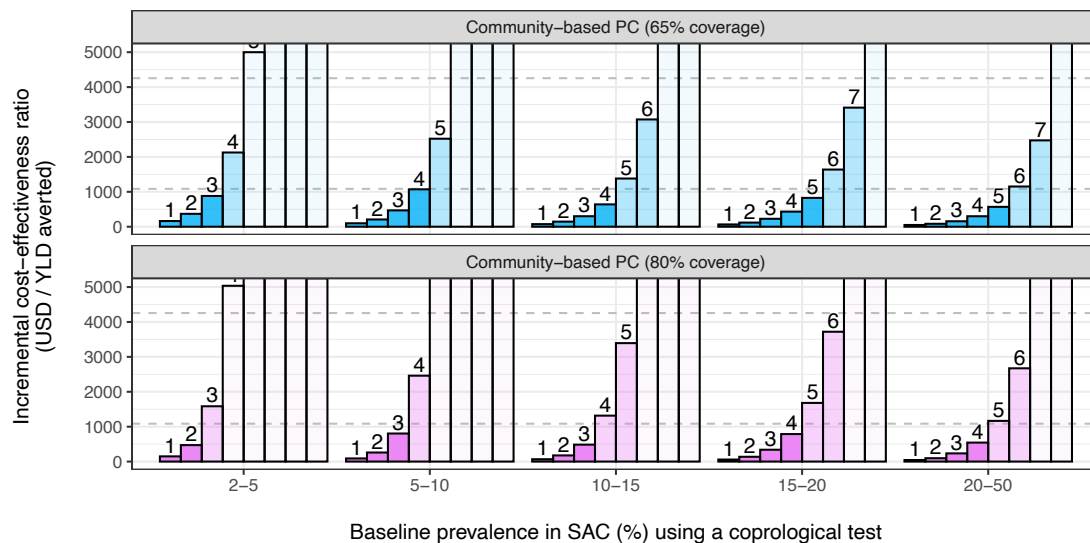
Supplemental Figure F. Incremental cost-effectiveness ratios (ICERs), based on years lived with disability or YLD, for increasing number of annual rounds of community-based preventive chemotherapy (PC). ICERs were calculated based on the cost of PC and the total number of disability-adjusted life-years lost over a 10-year period, applying a 3% discounting rate to both cost and effects. The number over each bar indicates the number of PC rounds, where the colour of bars indicates whether the ICER for that number of PC rounds was under the average gross domestic product (GDP) for low-income countries (US$1,085, lower dashed line) or under the average GDP of lower middle-income countries (US$4,255, upper dashed line), or over. 39 ICERs greater than US$5,000 are capped at the top of each panel. Note that ICERs may be underestimated for the shortest PC program durations. This is because an average cost per treatment (calculated for a 10-year period) was applied to all PC program durations, not considering a potential concentration of costs at the start of PC programs. This also means that the ICERs for longer program durations may be lower than presented here.
