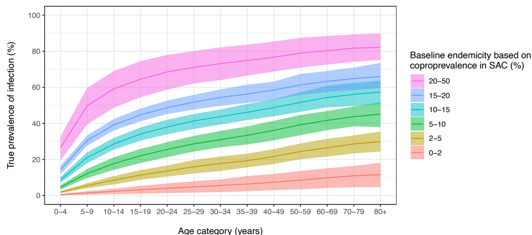
Figure 2. Model-predicted baseline age patterns in prevalence of infection, stratified by endemicity of Strongyloides stercoralis . Lines and ribbons represent the mean and 60%-confidence interval of simulated populations of 10,000 people. Age patterns are stratified by baseline endemicity (colours) as measured in school age children (SAC) with a coprological test (50% sensitivity).
