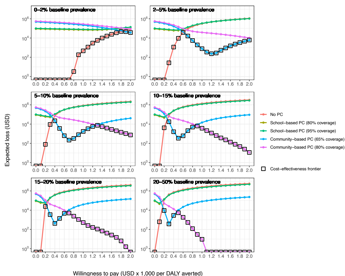
Figure 4. Expected loss in US dollars as a function of willingness to pay (WTP) per DALY averted in a population of 100,000 individuals. For a given WTP, the most cost-effective strategy is the one that minimises the expected loss (indicated with black open squares). Cost of distribution of ivermectin was assumed to be as estimated for preventive chemotherapy against soil-transmitted helminths in Dak Lak province, Vietnam. 33 The line for school-based PC at 80% coverage is largely hidden behind the line for school-based PC at 95% coverage. Panels represent settings with different baseline infection prevalence in school age children, as measured with a coprological test (assuming 50% sensitivity and 100% specificity). Bullets on the horizontal axis indicate situations where the expected loss was zero, meaning that a strategy always produced the highest net benefits and was the most cost-effective across all simulated populations and across the range of uncertainty about cost and health impact.
