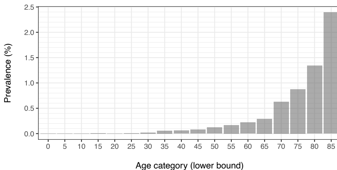
Supplemental Figure B. Simulated prevalence of immune-compromised states in a strongyloidiasis-free population. The prevalence pattern is result of the assumption that the average incidence of immune-compromised states per life-year is such that the 80-year-life-time risk is 2.5% and that the immune-compromised state develops at 95% of the total strongyloidiasis-free life expectancy. Prevalence for ages 80+ was not exactly 2.5% due to stochastic variation, which was considerable for higher age groups due to a relatively low number of individuals. The overall prevalence of immune-compromised states in the plotted population was 0.1%. The figure is based on a one-time simulation of a population of 500 thousand people.
