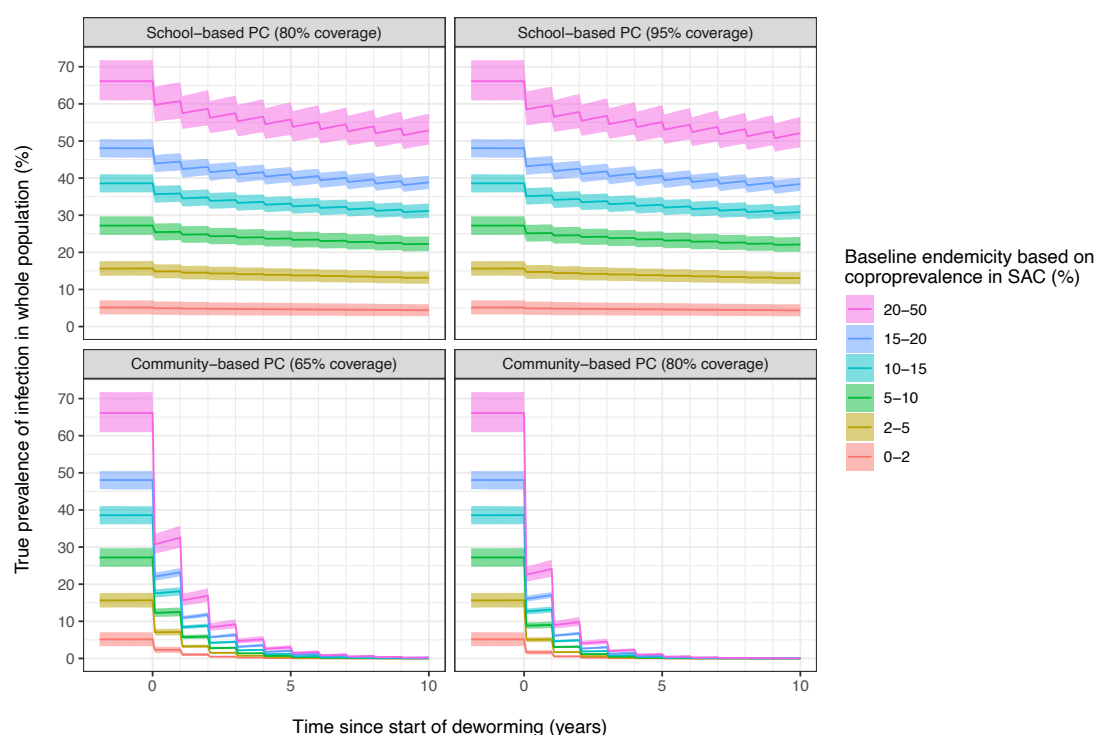
Figure 3. Model-predicted impact of different preventive chemotherapy (PC) strategies on true prevalence of Strongyloides stercoralis in a population of 100,000 people. Trends are stratified by baseline endemicity (colours) as measured in school age children (SAC) with a coprological test (50% sensitivity, 100% specificity). Lines and ribbons represent the mean and 95%-confidence interval of predicted values per endemicity category.
