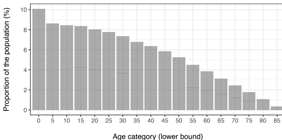
Supplemental Figure A. Age distribution of simulated populations, using demographic and mortality data from sub-Saharan Africa in 2000. In countries that have already (partly) gone through the first and/or second demographic transition (first = reduced child mortality; second = reduced birth rate), populations may consist of relatively more adults than we simulate here. As such, the demography we simulate somewhat favours school-based deworming as a relatively larger proportion of the population is captured by such a strategy.
