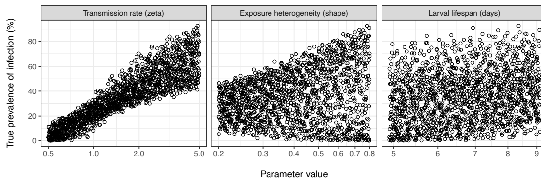
Supplemental Figure C. Simulated baseline prevalence of infection as a function of transmission conditions. Each point represents one of 1,500 random transmission conditions. Transmission conditions were defined in terms of the overall transmission rate (left), the level of exposure heterogeneity (middle; lower parameter values represent higher heterogeneity), and the average lifespan of free-living infective larvae in the environment (right). Plotted prevalences represent prevalence in the entire population as if measured by a 100% sensitive and 100% specific diagnostic tool.
