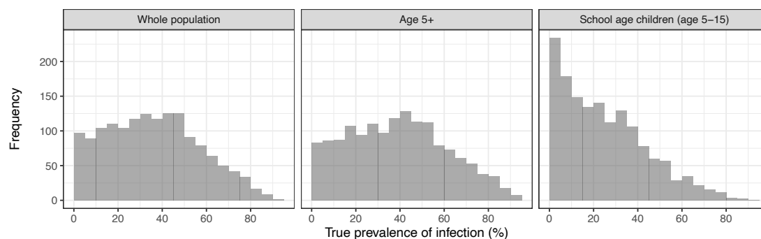
Supplemental Figure D. Histogram of simulated baseline prevalence of infection by age group. Each histogram represents 1,500 random transmission conditions (i.e., all bars add up to 1,500). Simulated baseline prevalences represent prevalence as if measured by a 100% sensitive and 100% specific diagnostic tool, and are shown for three age groups.
