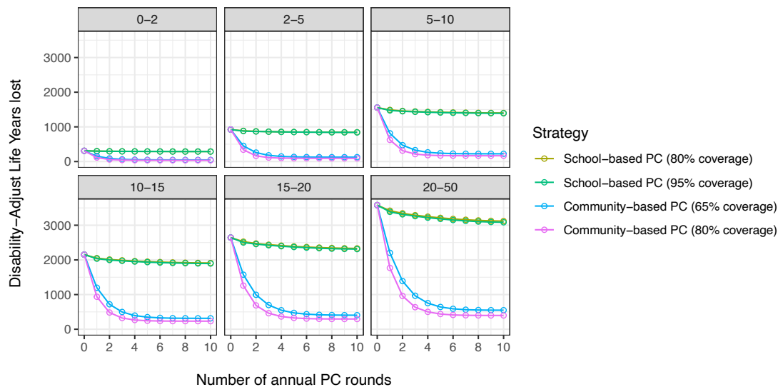
Supplemental Figure E. Disability-adjusted life-years (DALYs) lost due to strongyloidiasis over 10 years under different scenarios for the number of annual preventive chemotherapy (PC) rounds. Panels represent different endemicity scenarios; panel labels indicate the baseline prevalence of infection (%) in school age children, as measured by a coprological test with 50% sensitivity and 100% specificity. Colours indicate different PC strategies in terms of target population and achieved coverage.
