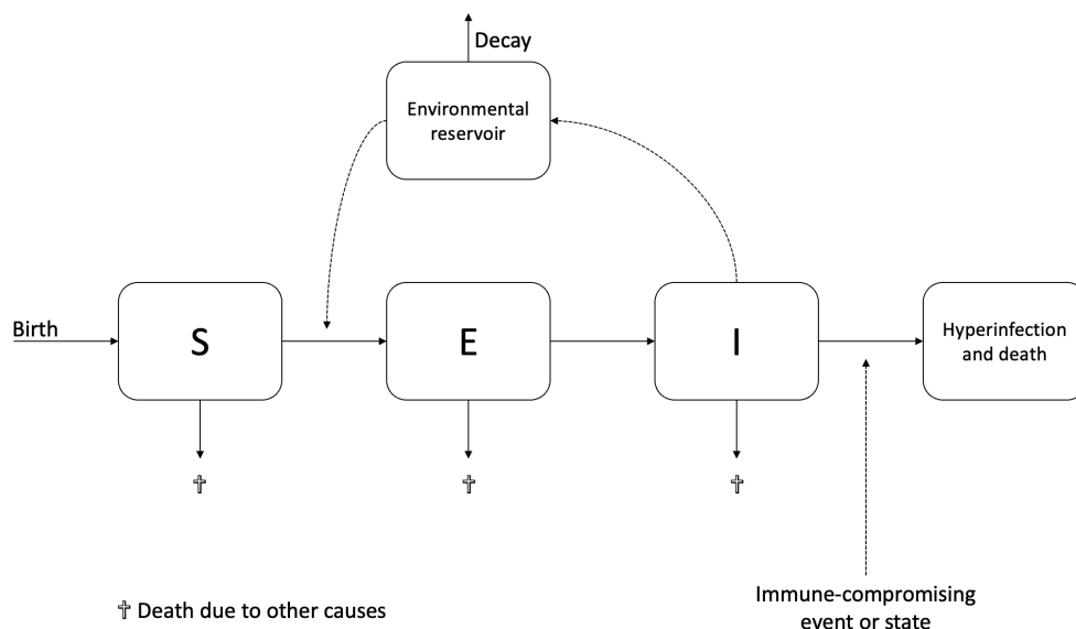
Figure 1. Schematic representation of an SEI model for Strongyloides stercoralis transmission. The model was implemented in a stochastic individual-based framework which explicitly includes age structure with a susceptible (S), exposed (E), and infectious (I) stage, along with an environmental reservoir. We account for risk of hyperinfection and death upon immunosuppression.
