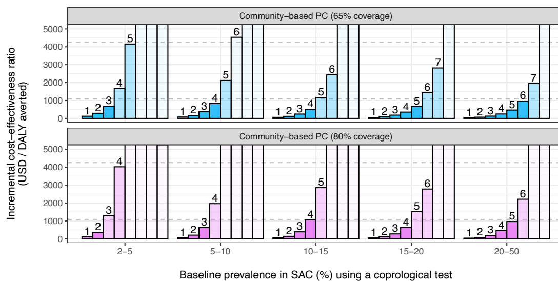
Figure 5. Incremental cost-effectiveness ratios (ICERs) for increasing number of annual rounds of community-based preventive chemotherapy (PC). The number over each bar indicates the number of PC rounds, where the colour of bars indicates whether the ICER for that number of PC rounds was under the average gross domestic product (GDP) for low-income countries (US$1,085, lower dashed line) or under the average GDP of lower middle-income countries (US$4,255, upper dashed line), or over. 39 ICERs greater than US$5,000 are capped at the top of each panel. Note that ICERs may be underestimated for the shortest PC program durations. This is because an average cost per treatment (calculated for a 10-year period) was applied to all PC program durations, not considering a potential concentration of costs at the start of PC programs due to initial start-up costs. This also means that the ICERs for longer program durations over-estimated somewhat.
