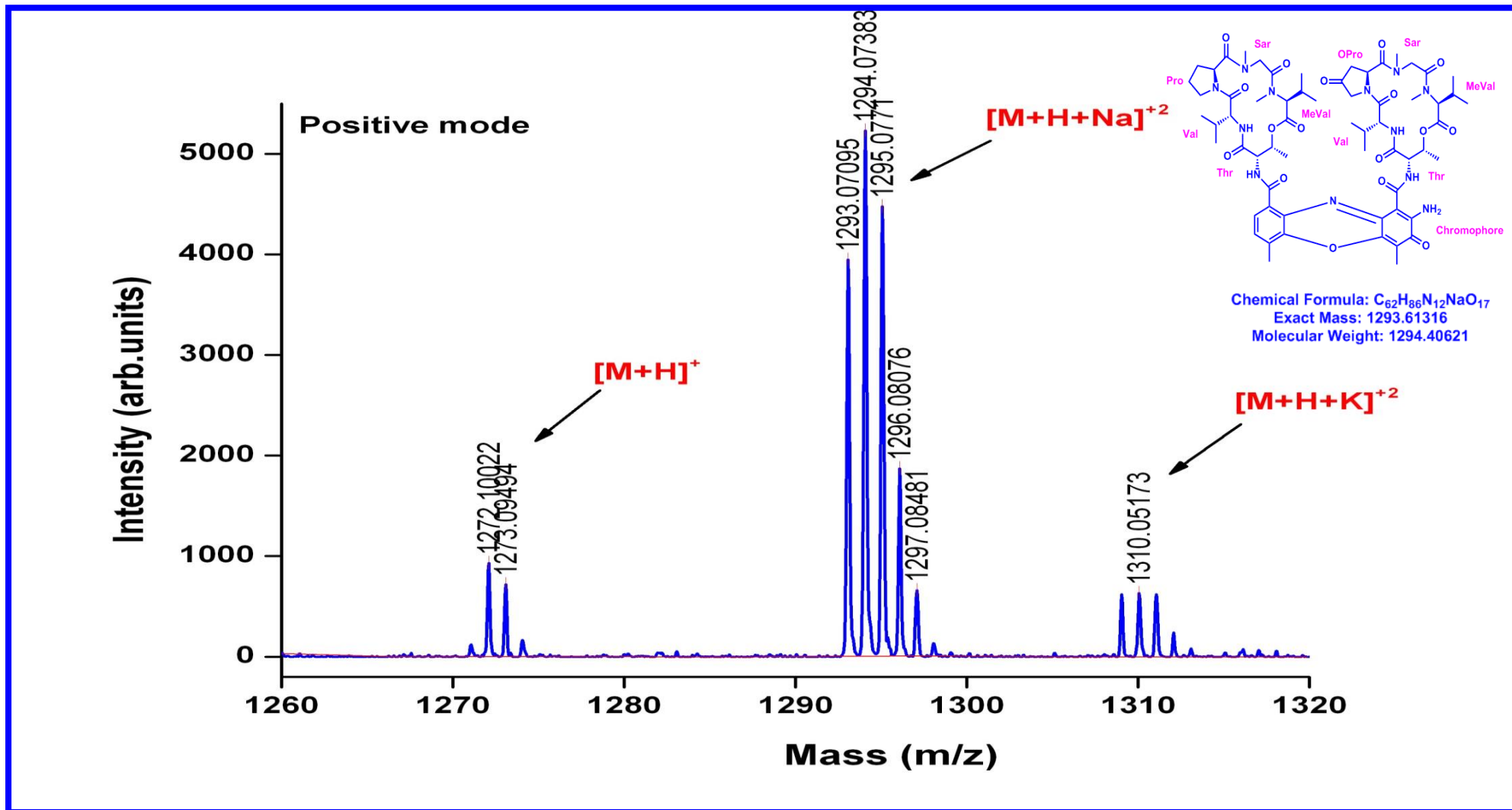
Figure S71. Expansion of MALDI-TOF MS Spectrum of Transitymycin (R1) (Molecular ion peak) (positive mode)
