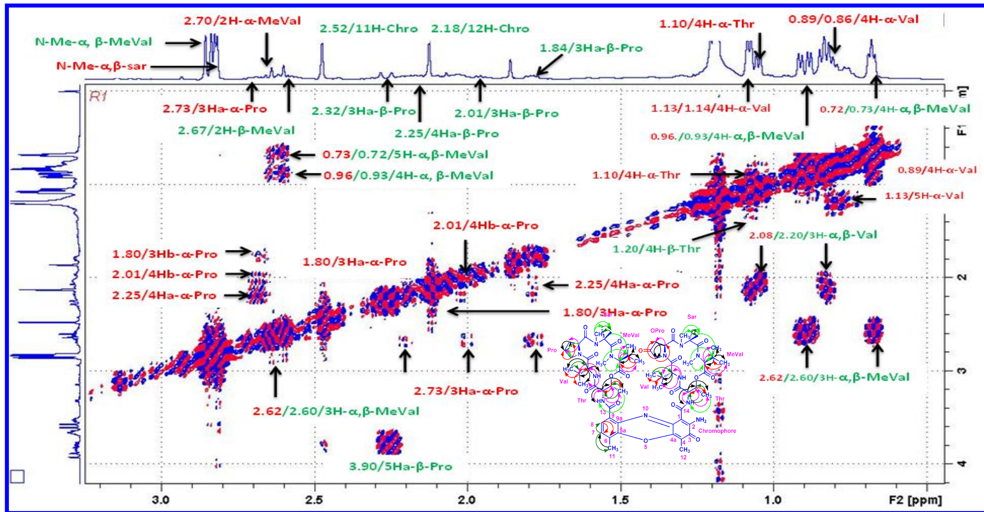
Figure S45. Expansion of TOCSY (500 MHz, CDCl 3 ) Spectrum of Transitycin (R1)
