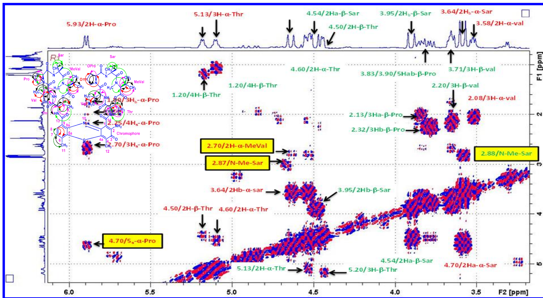
Figure S44. Expansion of TOCSY (500 MHz, CDCl 3 ) Spectrum of Transitmycin (R1)
