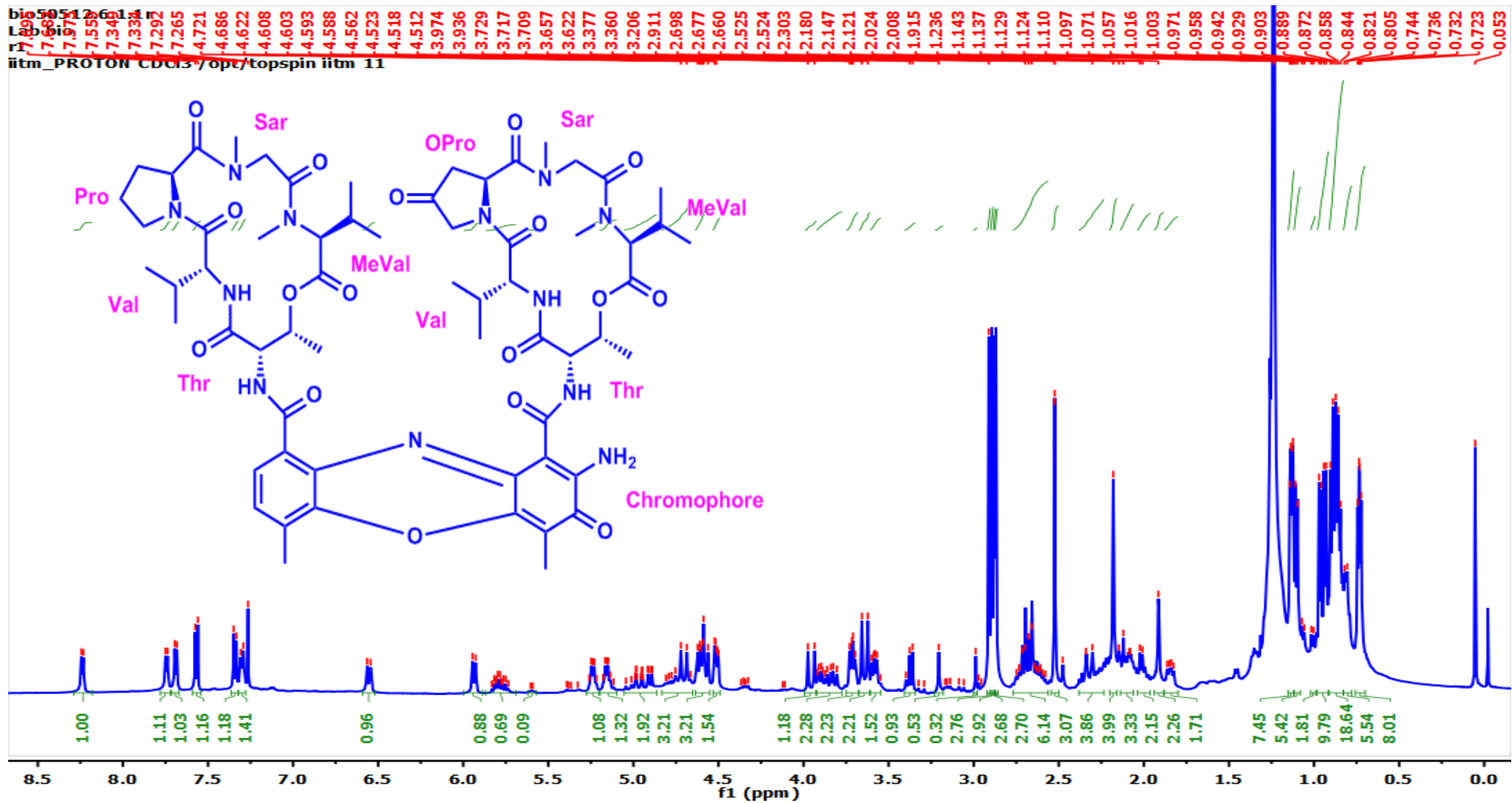
Figure S14. ^1\text{H-NMR} (500 MHz, \text{CDCl}_3 ) Spectrum of Transimycin (R1)
