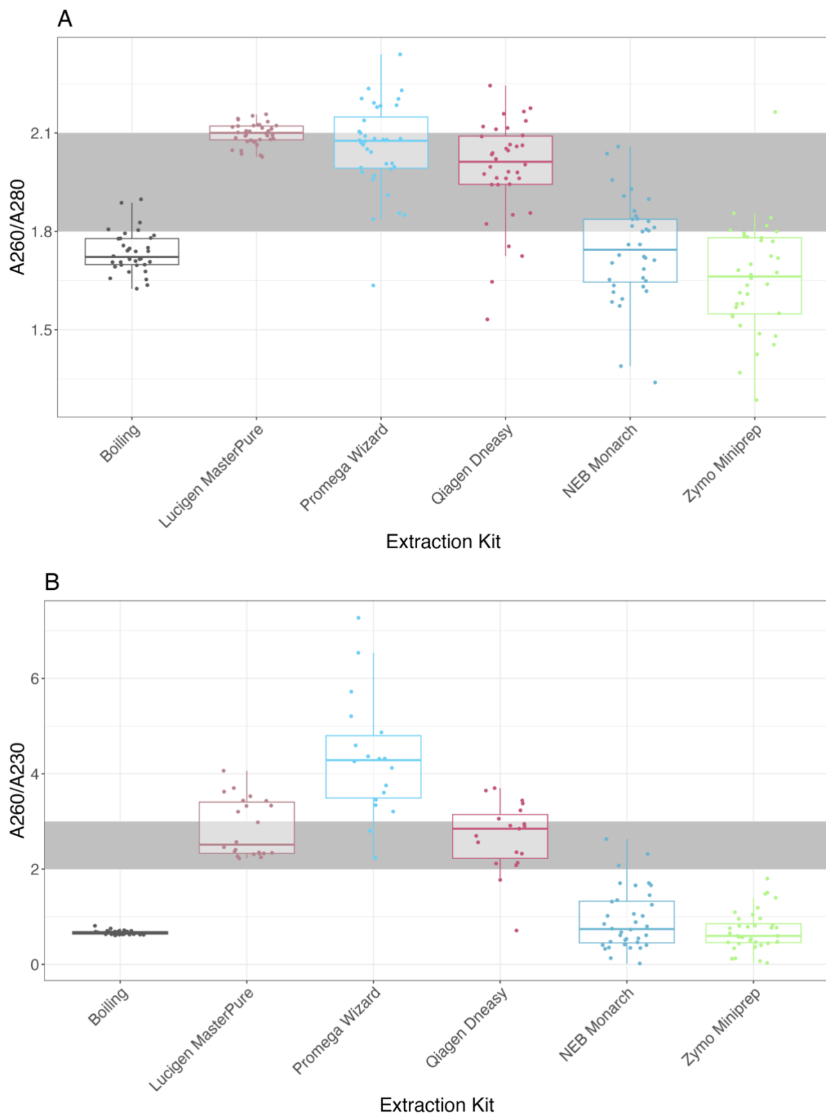
Figure 4 Absorbance ratios (A) A260/280 and (B) A260/230 indicating the presence of contamination and quality of DNA, respectively, of the extracted DNA extracted using six extraction methods. Technical (each sample extracted in
