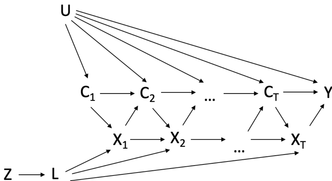
Figure 3. Causal diagram depicting time-varying confounders \{C_1, C_2, \dots, C_T\} affected by exposure ( X ), when the outcome ( Y ) is measured at the end of follow-up. \{X_1, X_2, \dots, X_T\} represent the exposure variables of interest measured at time points 1, 2, ..., T . \{C_1, C_2, \dots, C_T\} represent the potential confounders measured at time points 1, 2, ..., T , where it is assumed that C_T occurs just before X_T . In this diagram, Y is the outcome of interest, measured at the end of the study (at visit T + 1 ), and U is a set of unmeasured factors that influence \{C_1, C_2, \dots, C_T\} and Y (adapted from Daniel et al. (41)). L is the underlying liability to the exposure \{X_1, X_2, \dots, X_T\} . Z is a set of
