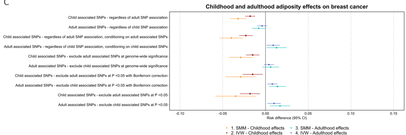
Figure 5. Causal risk difference estimates from univariable and multivariable MR using structural mean models (SMMs) and inverse variance weighted models (IVW) for childhood and adult adiposity and liability to childhood and adult adiposity, respectively, on the outcome measures listed. (A) Childhood and adult adiposity period effects on cardiovascular disease (CVD). (B) Childhood and adult adiposity period effects on Type 2 diabetes (T2D). (C) Childhood and adult adiposity period effects on breast cancer. Associated SNPs refers to strongly associated at genome wide significance ( P \leq 5 \times 10^{-8} ).
