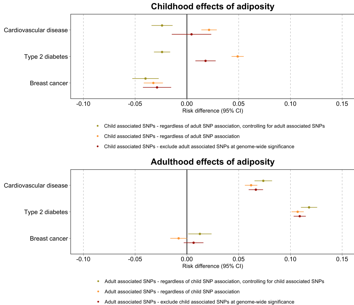
Figure 4. Causal risk difference estimates from univariable and multivariable MR using structural mean models (SMMs) for childhood and adulthood adiposity period effects on the outcome measures listed. Associated SNPs refers to strongly associated at genome wide significance ( P \leq 5 \times 10^{-8} ).
