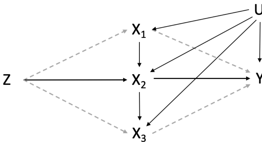
Figure 1. Causal diagram for instrumental variable analyses with one measured period ( X_2 ) (using instruments associated with three potential time periods) of an exposure. Z is a set of genetic variants associated with X_2 , Y is an outcome observed at one time only, X_1 and X_3 indicate potentially relevant periods that are unmeasured. U is a set of unobserved confounders of the exposure at each time period and the outcome. X_1 , X_2 , X_3 and Y are confounded by a set of unobserved confounders U . Dashed lines indicate paths via unmeasured exposures.
