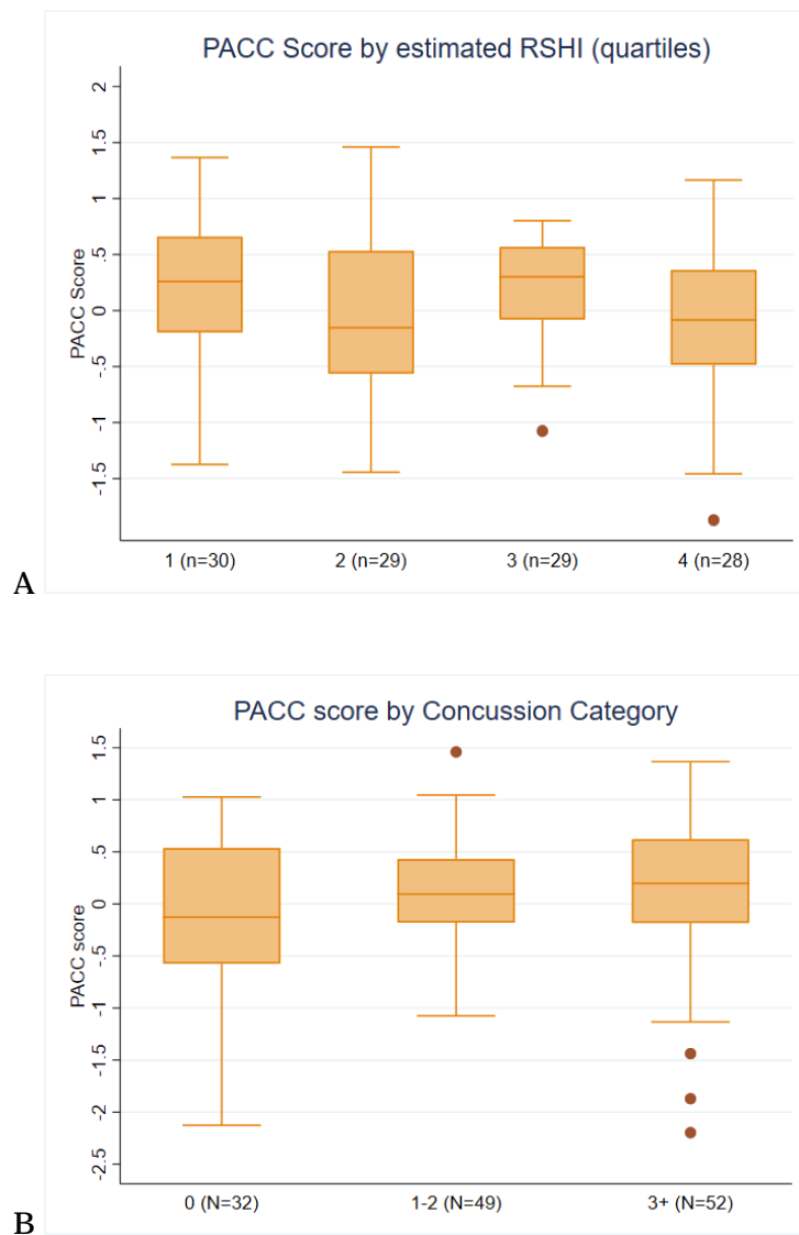
FIGURE 1: DISTRIBUTION OF PACC SCORES BY QUANTILES OF DISTRIBUTION OF ESTIMATED CUMULATIVE HEADING (A) AND BY CONCUSSION CATEGORIES (B)
