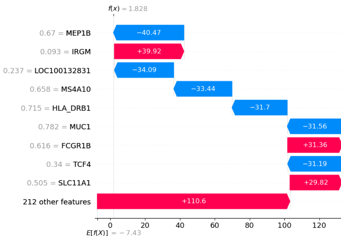
Figure 3: Waterfall plot for analysing model output for a single patient (Patient 260) for the “CD deep ulcer” disease subtype (using dependent features). Shown are contributions made from the top genes identified, alongside that of the remaining genes. The plot shows how the model output has hifted from the expected value E[f(z)] , where the model has no information about the features, to the actual output, f(x) (values are in log-odds space). Shown are some highly relevant genes, such as IRGM which is a negative regulator of IL1B as it suppresses NLRP3 inflammasome activation. It has a protective effect against gut inflammation in CD. IRGM has a relatively low normalised expression level of 0.093 for this patient, which would have little protective effect. This leads the model to predict a greater probability of CD with deep ulcer.
