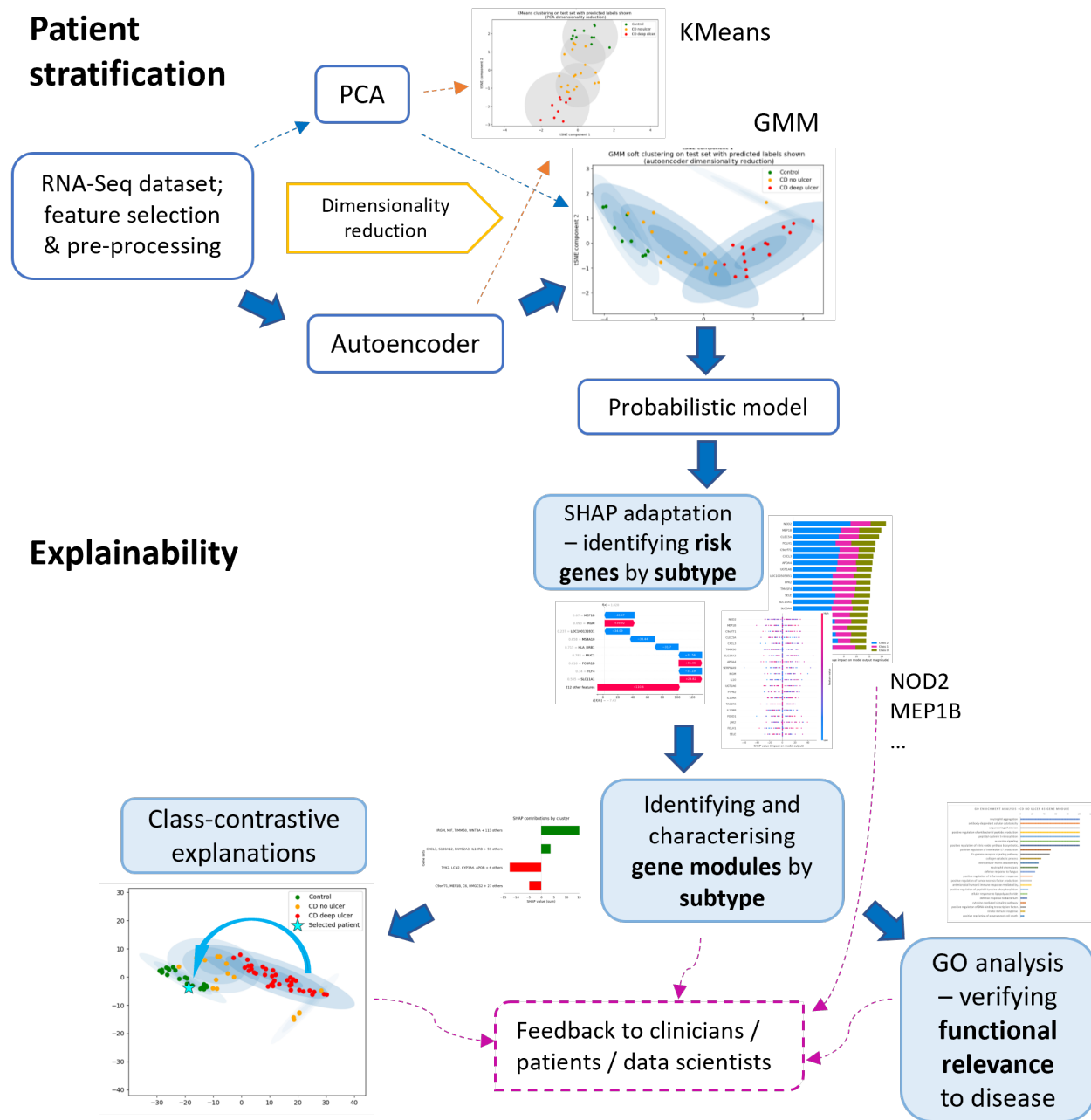
Figure 1: Overview of our computational framework. We identify genes and gene modules implicated in Crohn’s disease (CD) subtypes. Starting with RNA-Seq data, we perform feature selection and reduce dimensionality using PCA and an autoencoder. We then use a probabilistic model (Gaussian Mixture Model [GMM]) to cluster patients into disease subtypes (CD with deep ulcer, CD without deep ulcer and control). In order to explain our model we develop: 1. an extension of Shapley Additive Explanations (SHAP) to account for gene correlations, and 2. a class-contrastive technique to visually demonstrate the effect of changing gene expression on individual patients. We confirm these findings by referencing a variety of peer-reviewed studies and conducting a Gene Ontology (GO) enrichment analysis.
