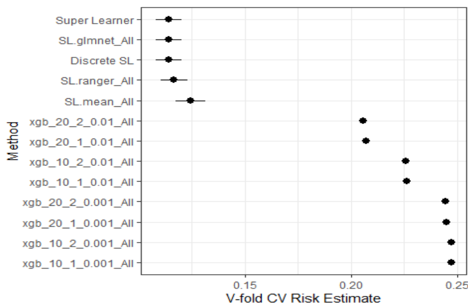
328 Figure 2: Plot the performance for the different supervised machine learning models fitted
