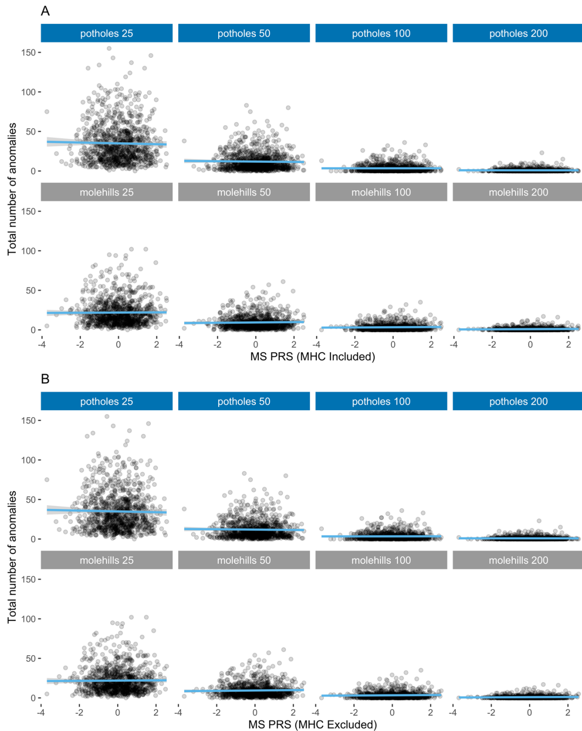
Figure 5: Association between the brain-wide number of potholes and molehills, per cluster size, and the MS PRS (SNP-association p -value threshold = 0.01) with A) MHC included B) MHC excluded.
