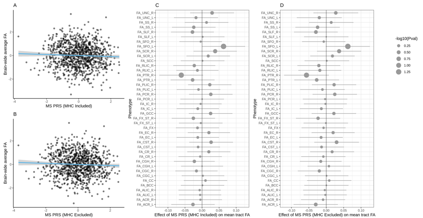
Figure 4: Association of MS PRS with brain-wide mean FA (3.A. – MHC included; 3.B. – MHC excluded) and MS PRS effect (beta value) on mean FA per brain tract (3.C. – MHC included; 3.D. – MHC excluded). The vertical lines in 3.C. and 3.D. represent 95 % confidence intervals. Tract name abbreviations are taken from the ENIGMA’s look-up table (Suppl. Table 2).
