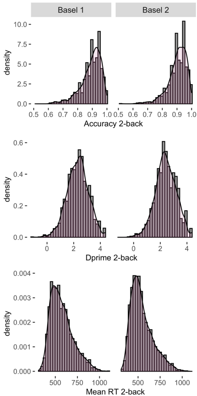
Figure 1: Distribution of participants' scores for accuracy, d prime and mean reaction time (RT) of the 2-back task, per subsample.
