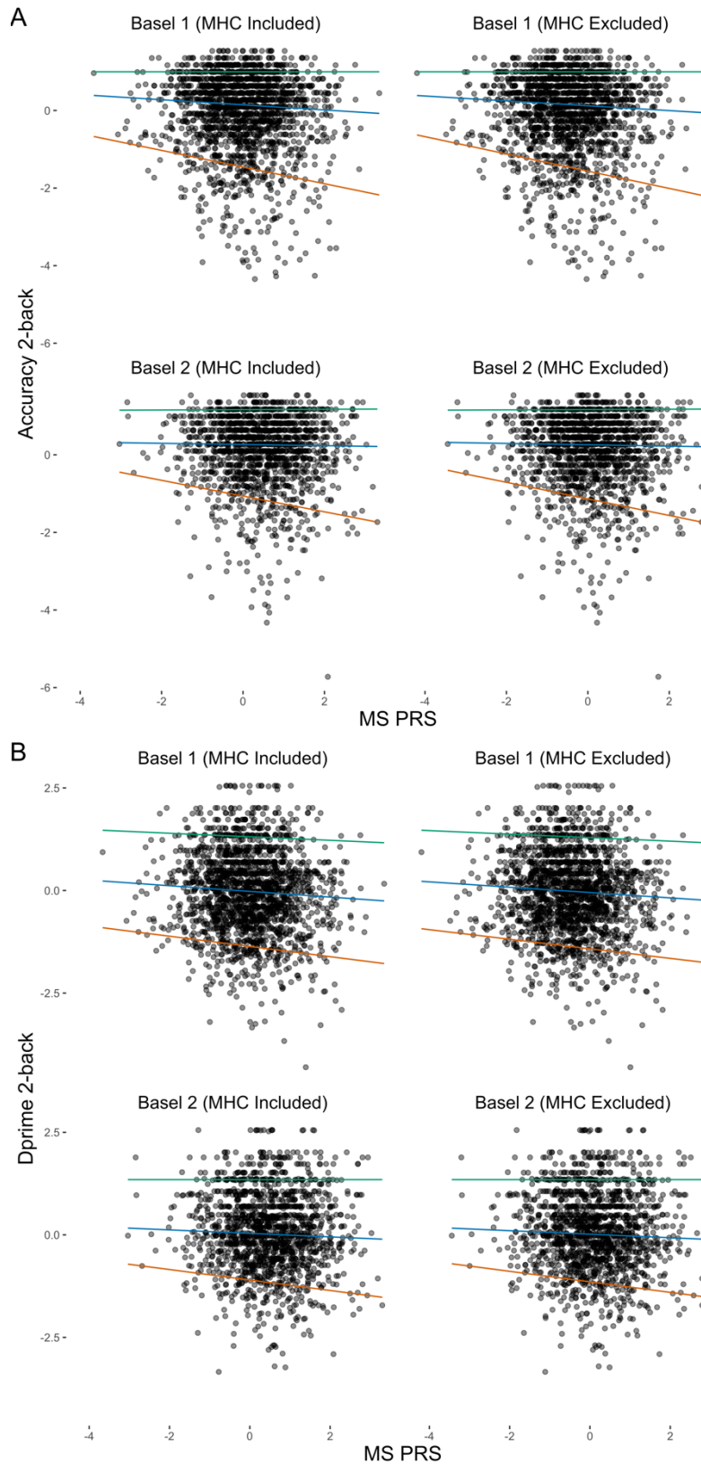
Figure 2: The association between the MS PRS at p-value threshold ( P_T ) of 0.05 and WM phenotypes A) 2-back accuracy and B) 2-back dprime in the Basel 1 and Basel 2 subsample. Each result is presented twice, for PRSs including and excluding the MHC). The 0.1, 0.5 and 0.9 quantile association is presented in red, blue and green colour, respectively.
