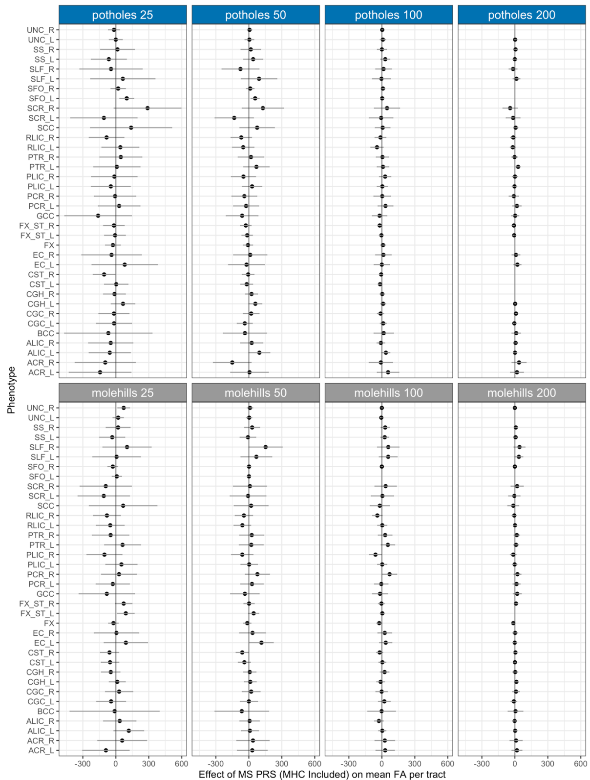
Figure 6: Association between the number of potholes and molehills within each brain tract, per cluster size, and the MS PRS (SNP-association p value threshold = 0.01), MHC included.
