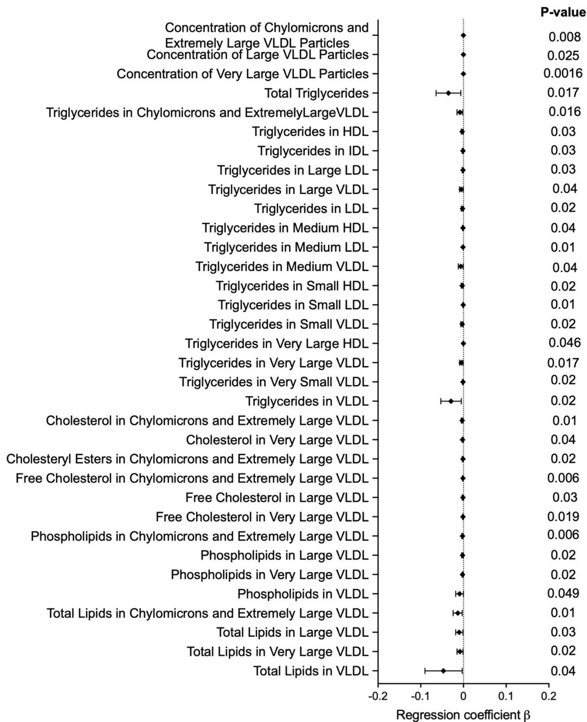
Figure 2: Forest plot demonstrating significant associations of rs3741596 with blood lipids traits.
