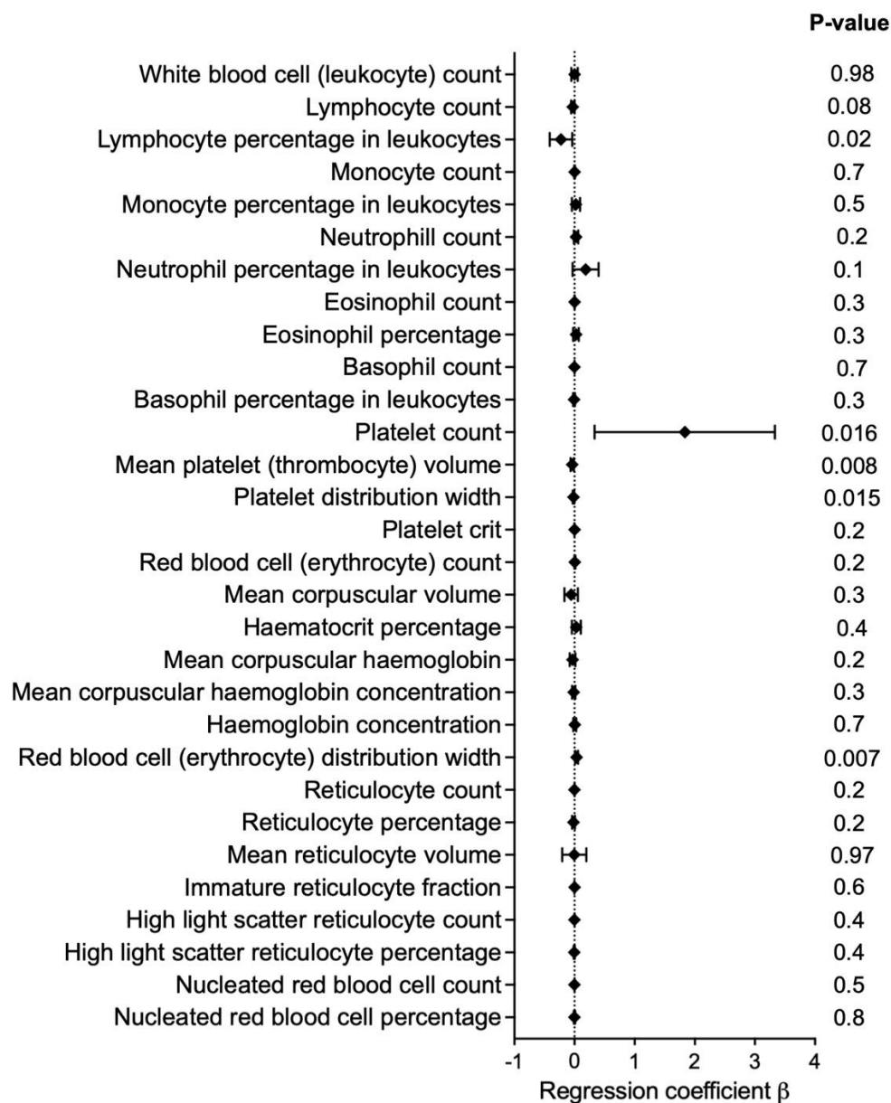
Figure 3: Forest plot demonstrating the associations of rs3741596 with blood cell traits.
