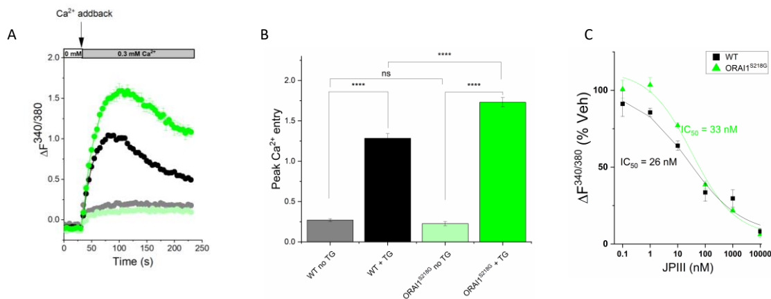
Figure 4: Functional characterisation of the ORAI1 S218G mutation in the Ca 2+ addback assay.
