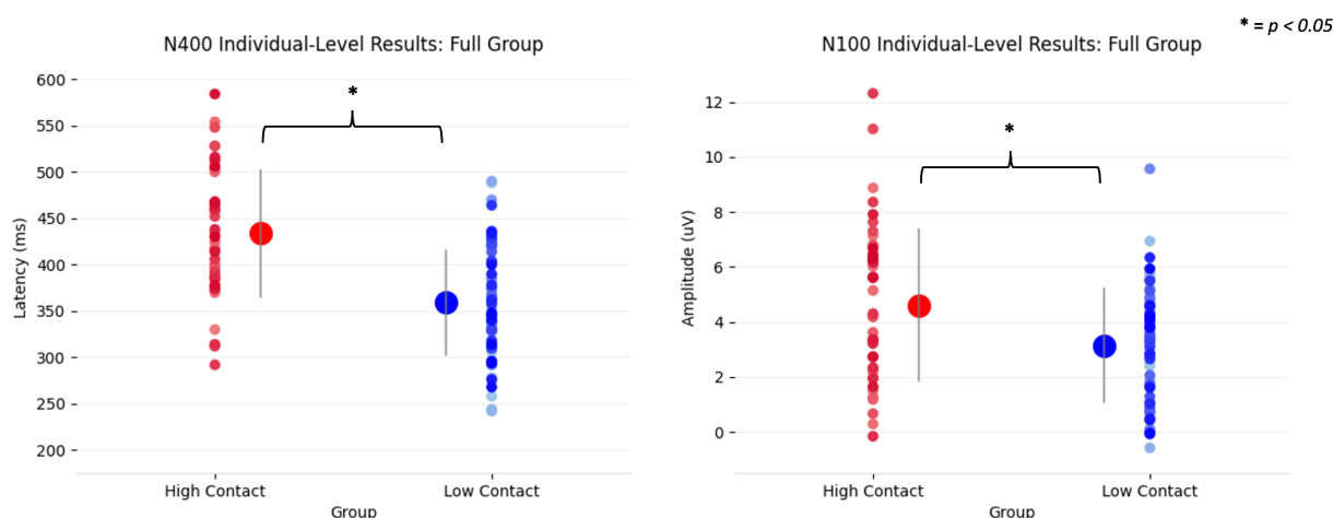
172 Figure 3: Individual scatter plot data, including group means and standard deviations (middle) showing a 173 significant N400 latency and N100 amplitude differences for high-contact (red) versus low-contact 174 (blue).
