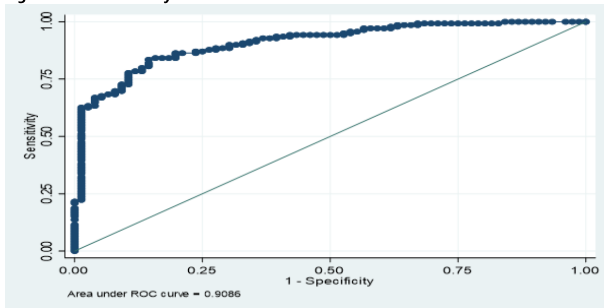
Figure 1: Model Validity
