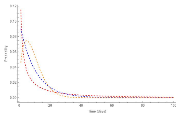
(b) Weibull distributions corresponding to the SIR Weibull model Eq (5.21) for \alpha = 0.5 (red dashed line), \alpha = 1 (blue dashed line), and \alpha = 1.5 (orange dashed line).
