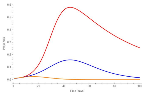
(a) Solutions of the SIR Weibull model Eq (5.21) considering \alpha = 0.5 (red line), \alpha = 1 (blue line), and \alpha = 1.5 (orange line).
