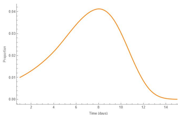
Figure 3: Numerical solution of the SIR with Weibull hazard function for \alpha = 5
