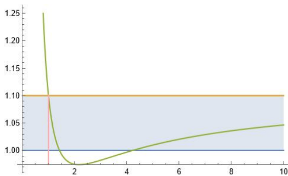
(a) Plot of expression (4.20) using the Weibull distribution (green line) as a function of \alpha (horizontal axis); R_0 = 1.1 for the SIR classical model (orange line), and R_0 = 1 (blue line). The pink line indicates the value \alpha = 1 for which R_0^W = R_0 = 1.1
