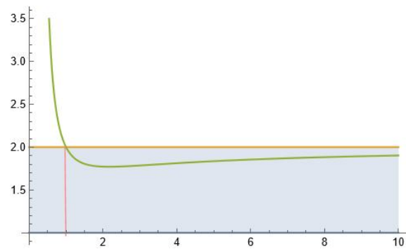
(b) Plot of expression (4.20) using the Weibull distribution (green line) as a function of \alpha (horizontal axis); R_0 = 2 for the SIR classical model (orange line), and R_0 = 1 (blue line). The pink line indicates the value \alpha = 1 for which R_0^W = R_0 = 2 .
