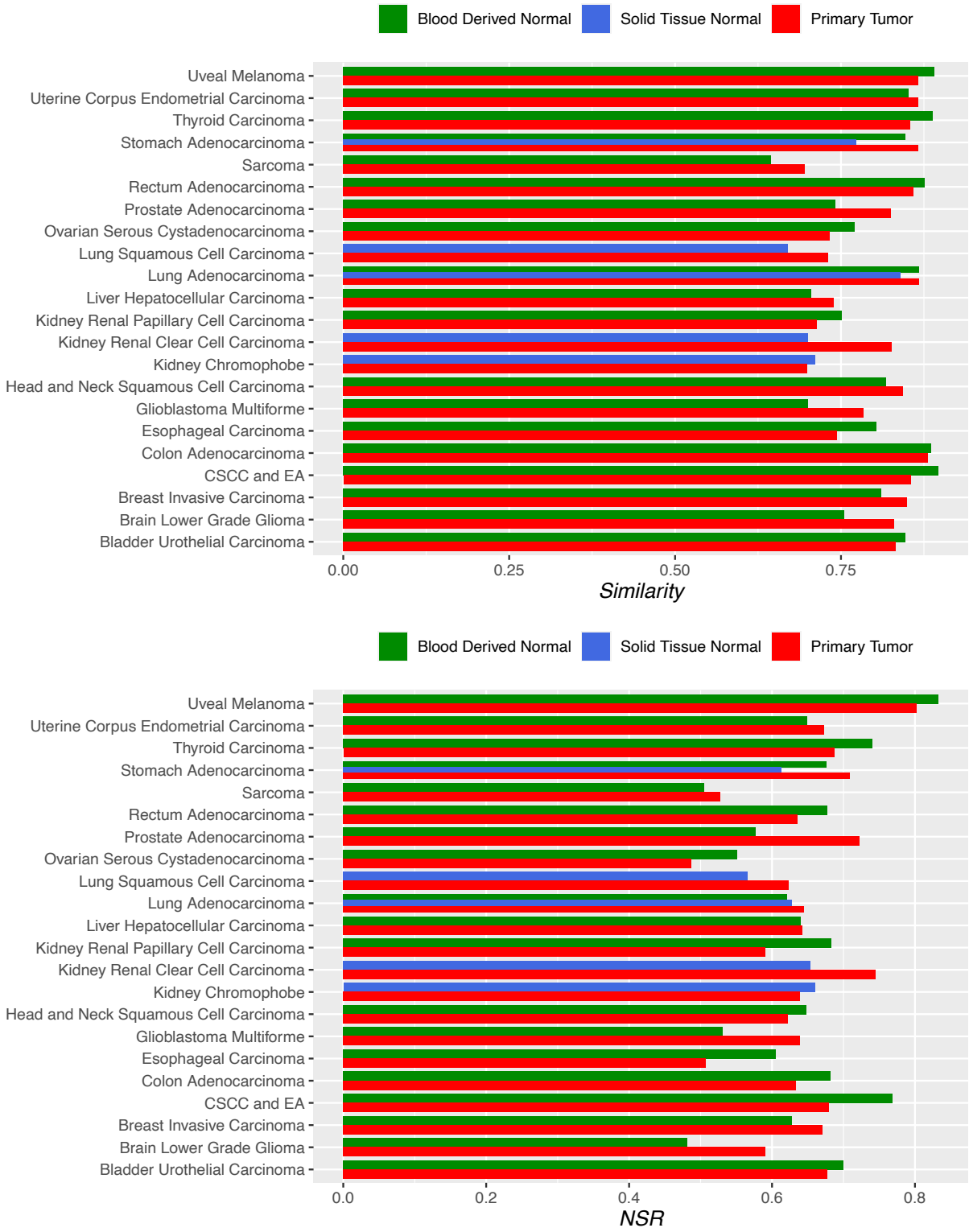
Fig 7. The comparisons of NSR (normalized stochasticity ratio) between PT (primary tumor), SN (solid tissue normal) and blood derived normal (B) for various cancer types with WGS datasets.
