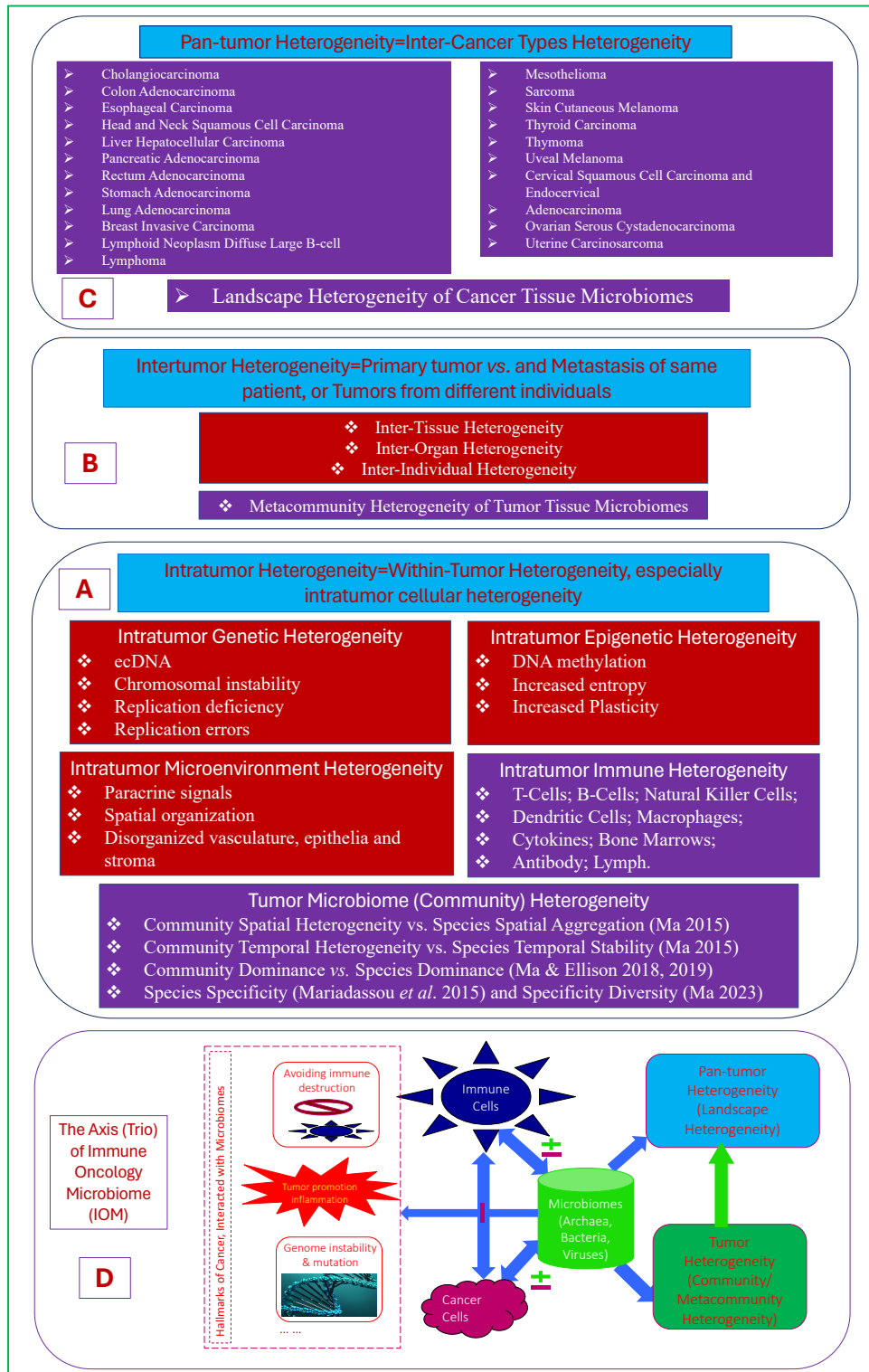
Fig 1. The relationships between tumor microbiome heterogeneity (TMH) and tumor heterogeneity (TH), as well as the IOM (immune-oncology-microbiome) trio. The pink blocks (e.g., tumor microbiome heterogeneity, pan-tumor heterogeneity) are new additions to the tumor heterogeneity concept defined by Marusyk et al. 2020). The middle blocks (B & C) are inspired by Figure (1) of Marusyk et al. (2020). The IOM trio (axis) follows Sepich-Poore et al. (2021).
