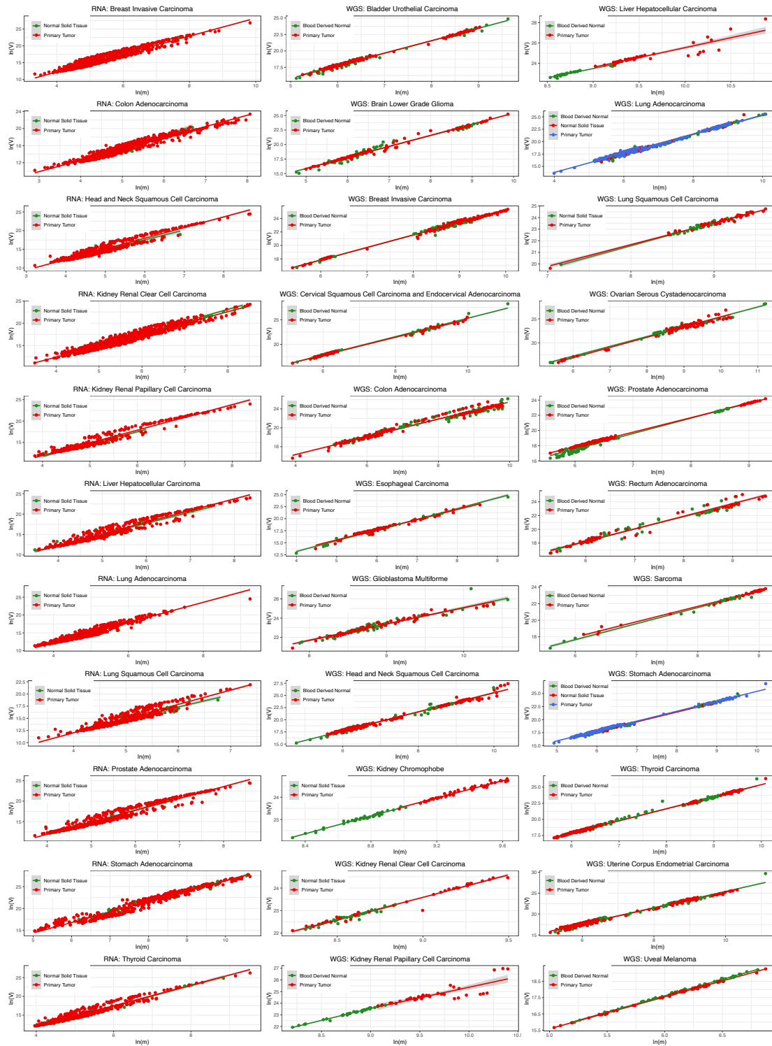
Fig 5. Fitting type-I TPLE (Taylor's power law) model for measuring community heterogeneity with cancer tissue microbiome datasets
