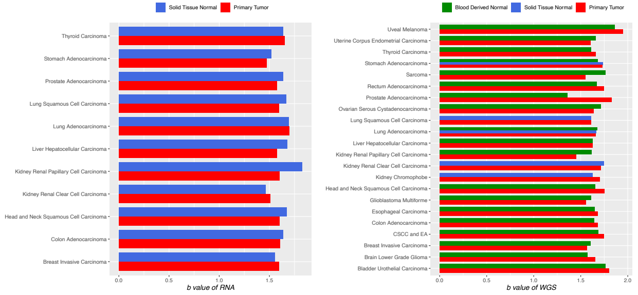
Fig 6. The tumor network heterogeneity scaling parameter ( b ) of TPLoN (Taylor's power law on network) built with RNA-Seq (the left) and WGS (the right) datasets.
