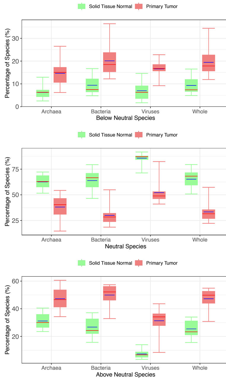
Figure 1. Box plots for percentages of below neutral, neutral and above neutral species for SNTM and PTM (Scheme I). The blue lines in box represent mean value across 11 types of cancer, and red lines are median. Standard bar charts showing the percentage of below neutral and above neutral species are significantly higher in the PTM than in the SNTM cohorts ( p < 0.001 ), while neutral species are significantly higher in the SNTM than in the PTM cohorts ( p < 0.001 ) (Table 1, Table S1, Table S2).
