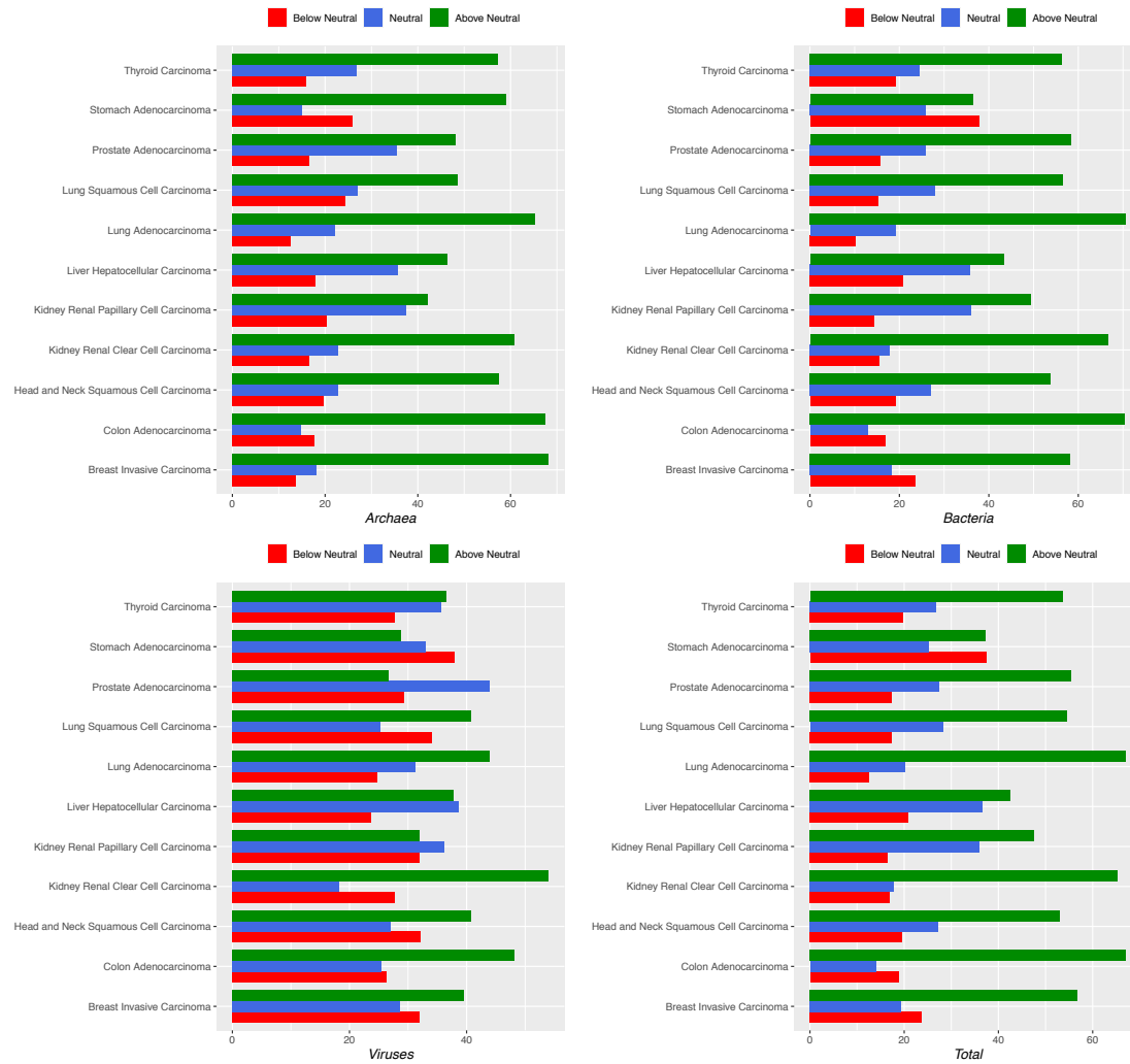
Figure 2. The percentage of below neutral species, neutral species, and above neutral species in PTM community. This neutral community model takes STNM community as source community and PTM as destination community.
