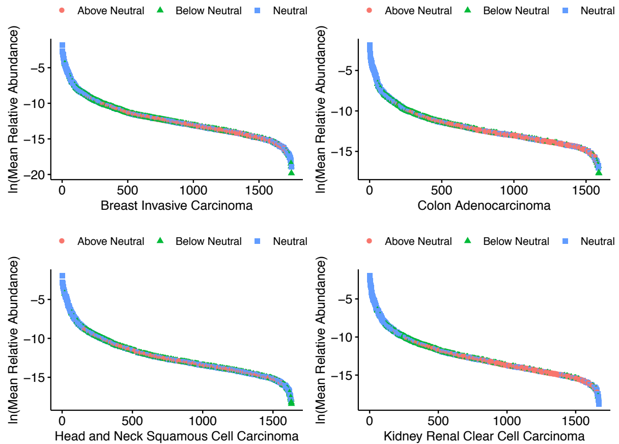
Figure 3. The species rank relative abundance of tumor tissue microbiomes. Neutral species are represented by blue points, below neutral species by green points, and above neutral species by red points. The y-axis represents relative abundance in nature logarithm of species; the x-axis represent species rank order in relative abundance.
