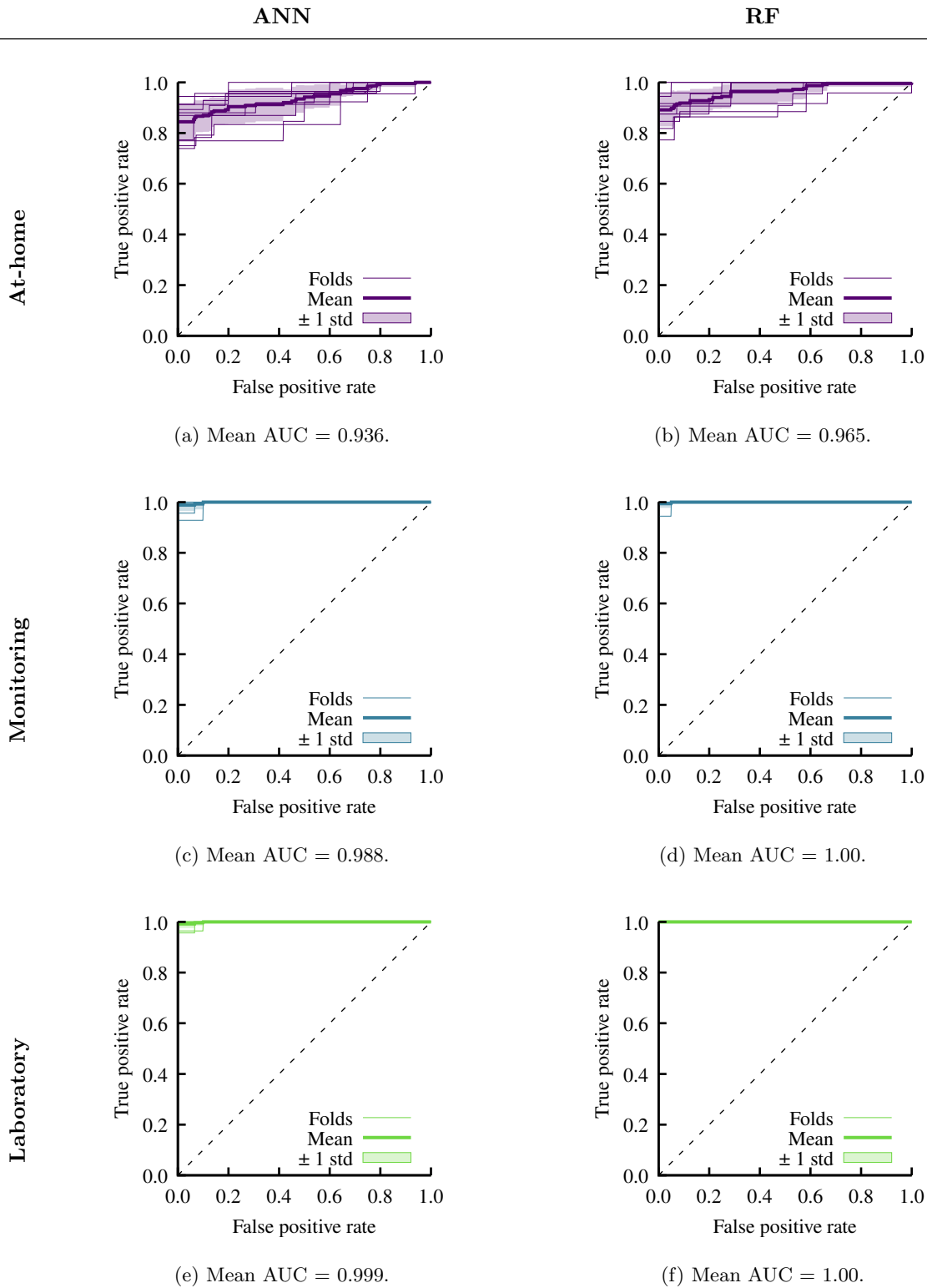
Fig. 1: CKD binary classification ROC curves with AUC values.
