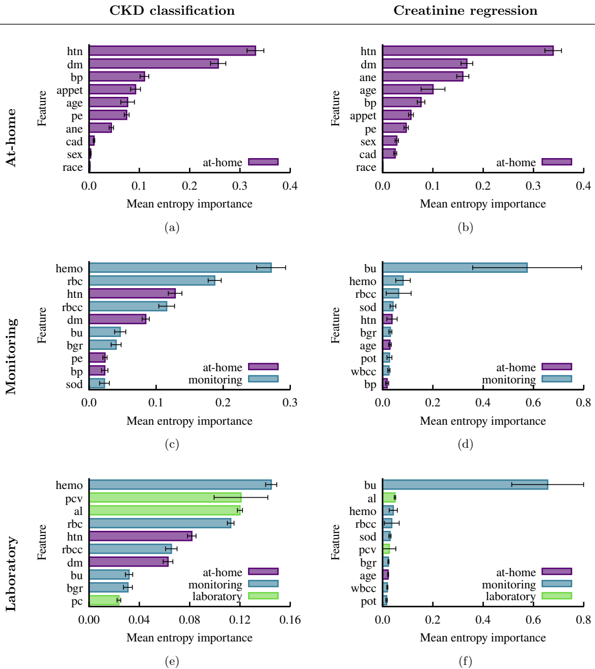
Fig. 2: Mean entropy importance for the six experiments extracted from RF. The error bars denote the standard deviation.
