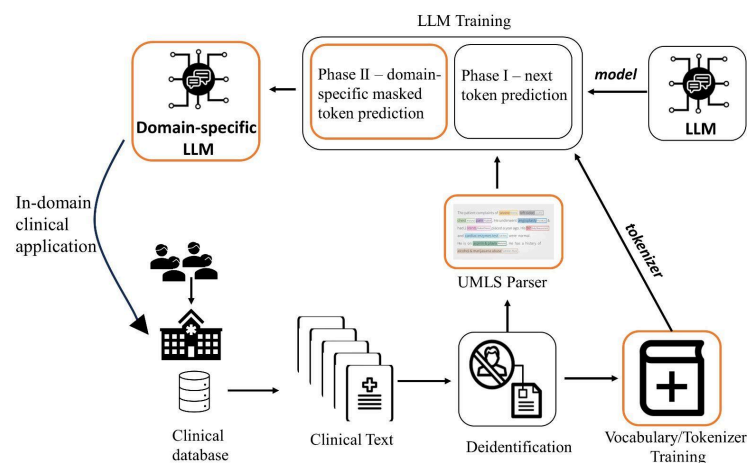
Figure 1: Domain-specific LLM training and application framework; Highlighted (orange-colored) modules indicate domain-specific modifications to LLM design framework.
